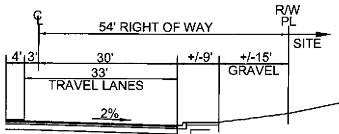
SECTION A SOUTH PROPERTY LINE WASHINGTON AVENUE INTERIM CONDITION
