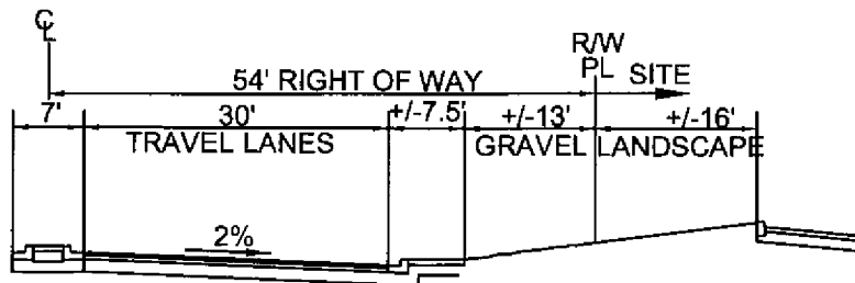
SECTION A SOUTH PROPERTY LINE WASHINGTON AVENUE INTERIM CONDITION
