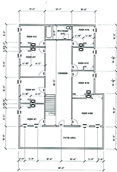
2 2ND FLOOR PLAN SHEET 1/8"
