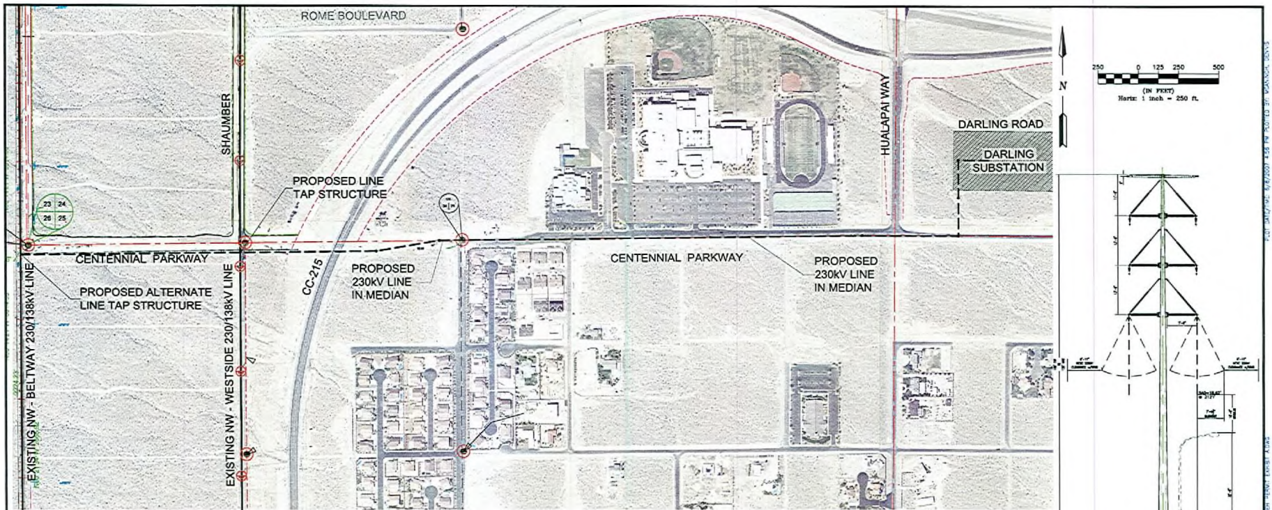
TYPICAL 230 kV STRUCTURE ROAD MEDIAN CONSTRUCTION
