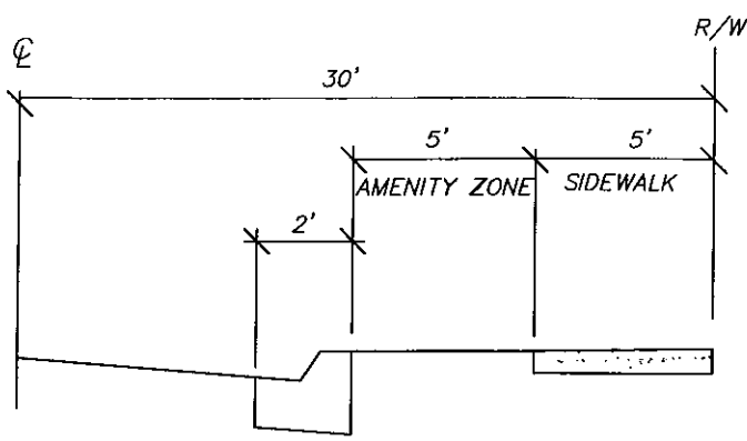
TYPICAL SECTION
