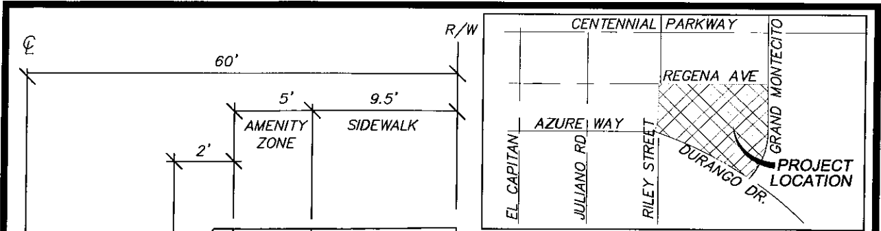
TYPICAL SECTION
