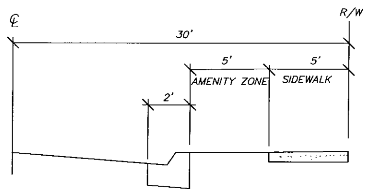
TYPICAL SECTION
