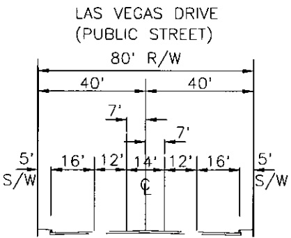
EXIST. TYPICAL STRIPING SECTION N.T.S.
