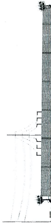
EAST WALL ELEVATION (View Looking West)
