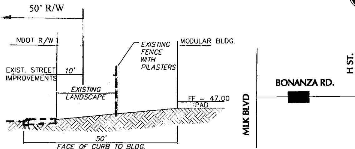
SECTION VIEW
