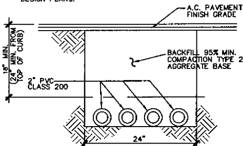
IRRIGATION SLEEVE DETAIL
