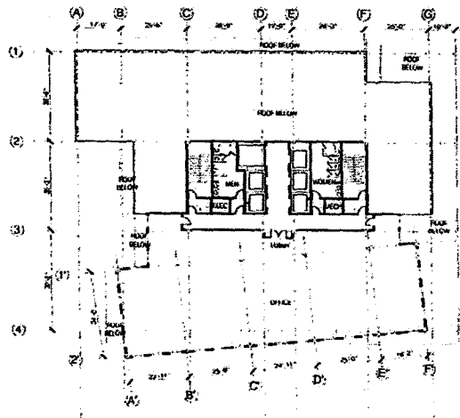
TENTH FLOOR PLAN
