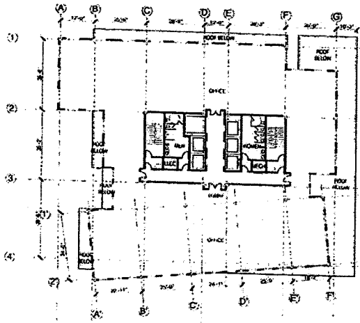
EIGHT FLOOR PLAN
