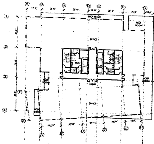
SIXTH FLOOR
