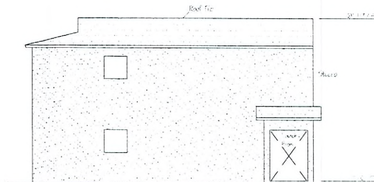
East Elevation 1/8" = 1'-0"
