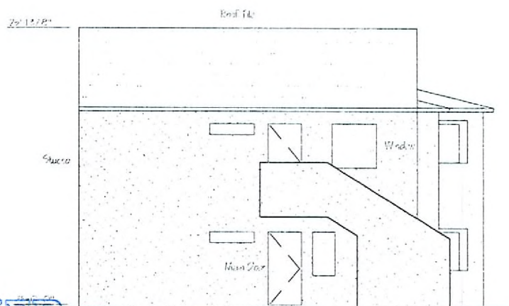
West Elevation 1/8" = 1'-0"
