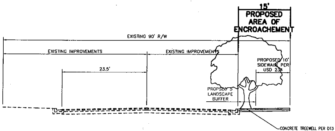
FREMONT STREET TYPICAL SECTION 'A'
