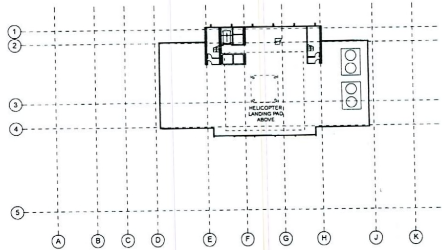
Roof Plan
