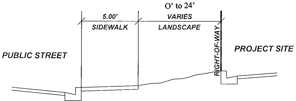
SECTION A-A TYPICAL LANDSCAPE ENCROACHMENT
