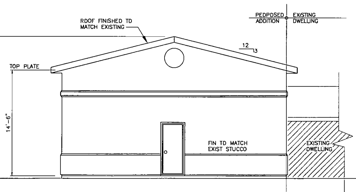
NORTH ELEVATION
