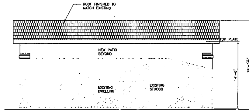
WEST ELEVATION
