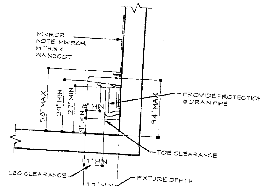
4 LEG CLEARANCES NOT TO SCALE
