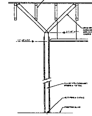
6. INTERIOR WALL DETAIL 1/4" = 1'-0"
