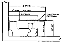
3. WATER CLOSET SIDE VIEW NOT TO SCALE
