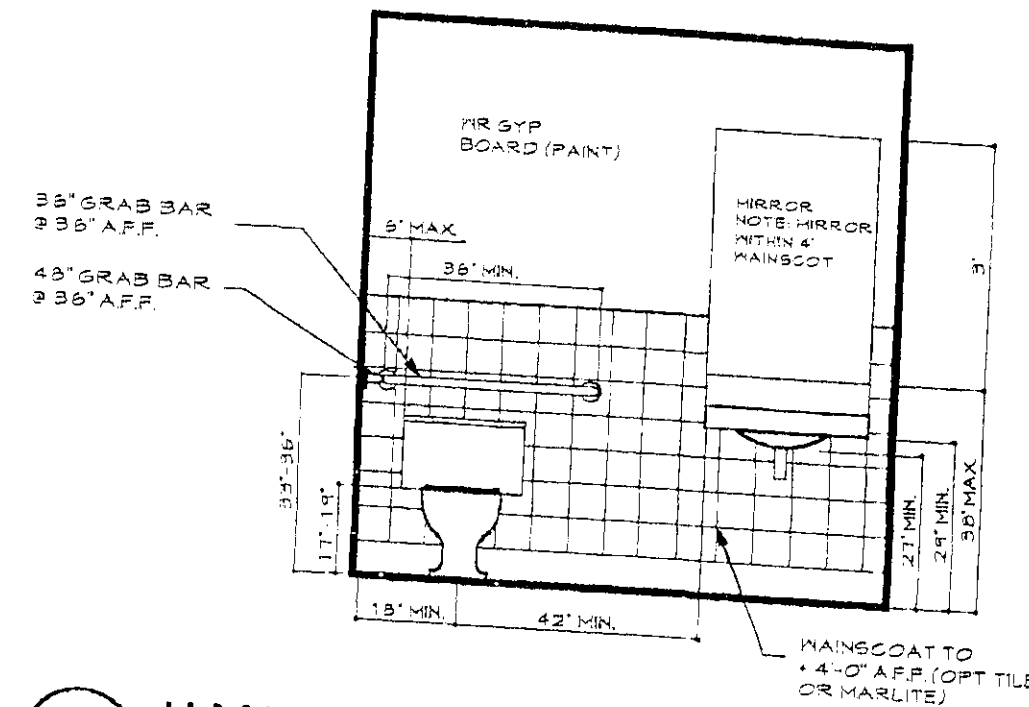
2 HANDICAP BATHROOM ELEVATION NOT TO SCALE
