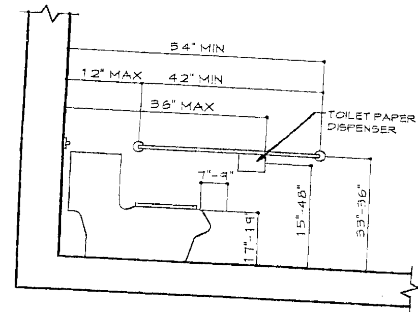
3 WATER CLOSET SIDE VIEW NOT TO SCALE
