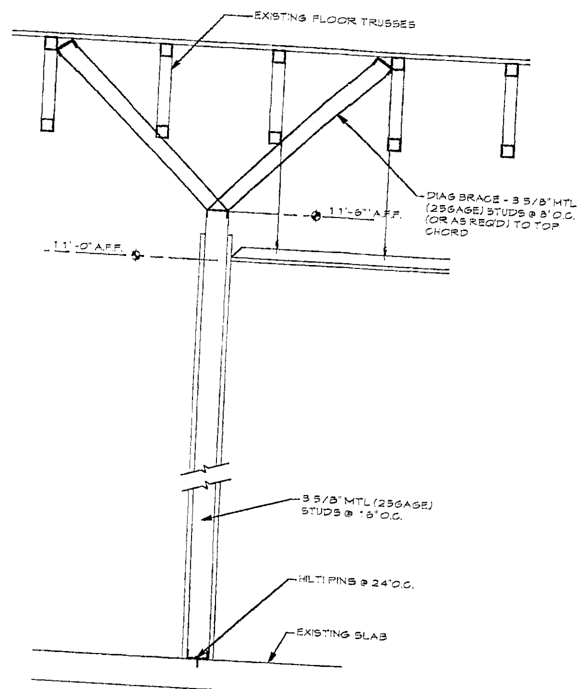
6 INTERIOR WALL DETAIL NTS
