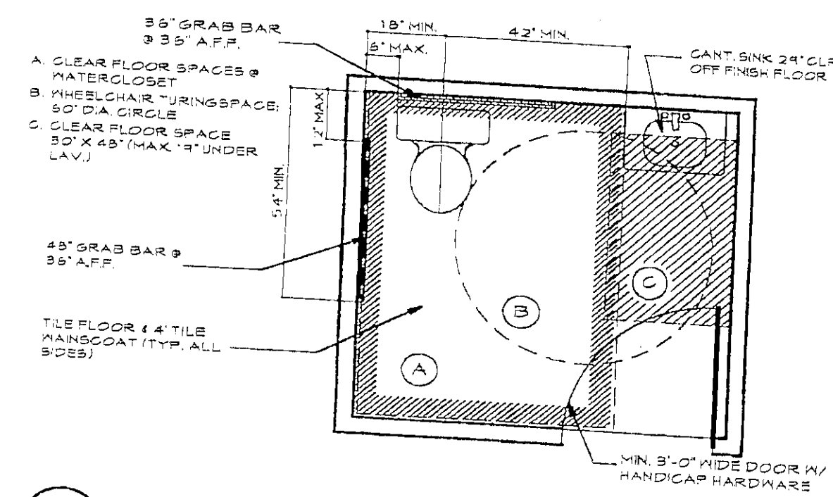
1 HANDICAP RESTROOM NOT TO SCALE 10" ET PROVIDE ELECTRIC EXHAUST FAN (TYP. ALL RESTROOMS)
