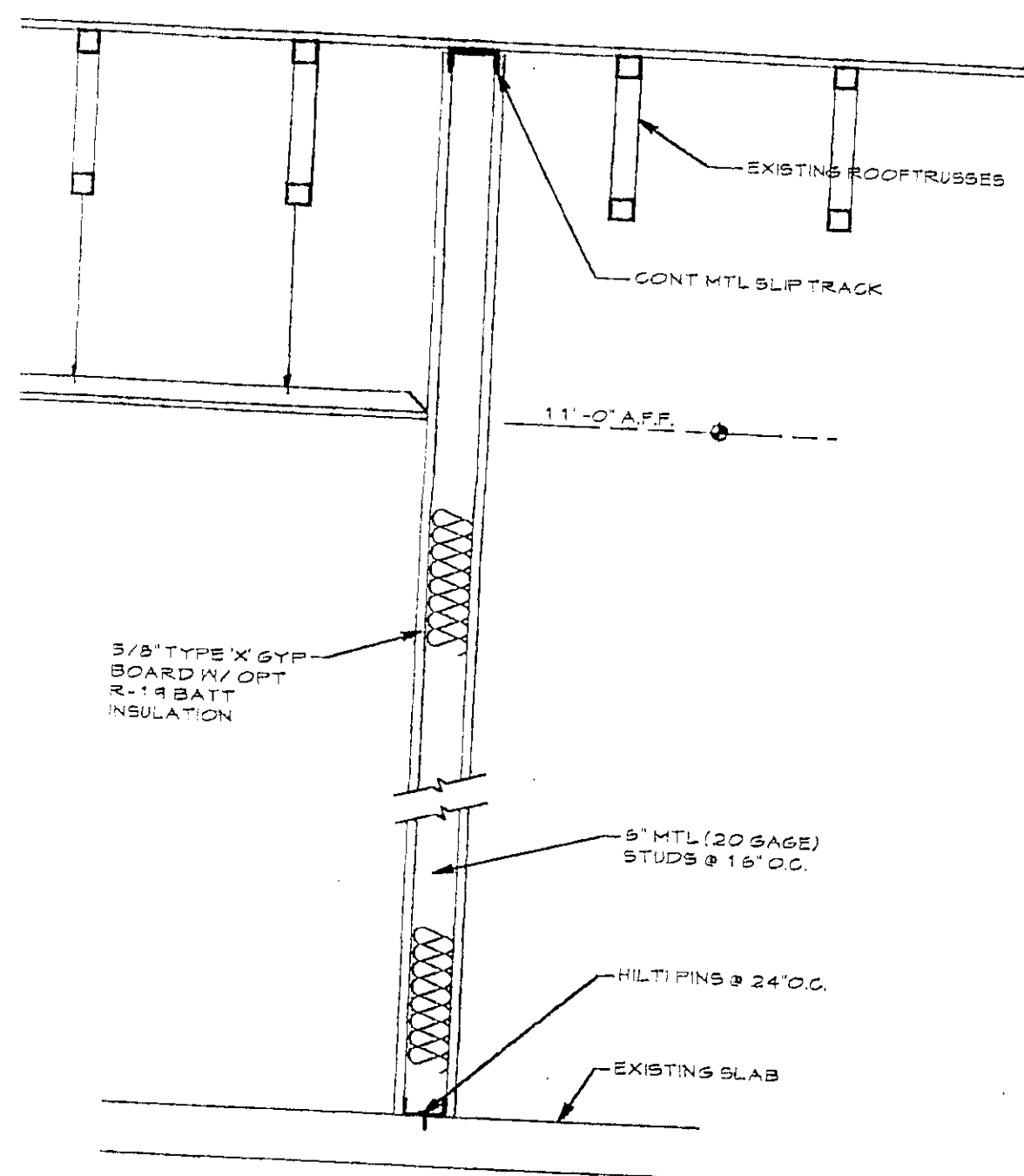
5 INTERIOR WALL DETAIL 1 HR EXISTING WALL NTS
