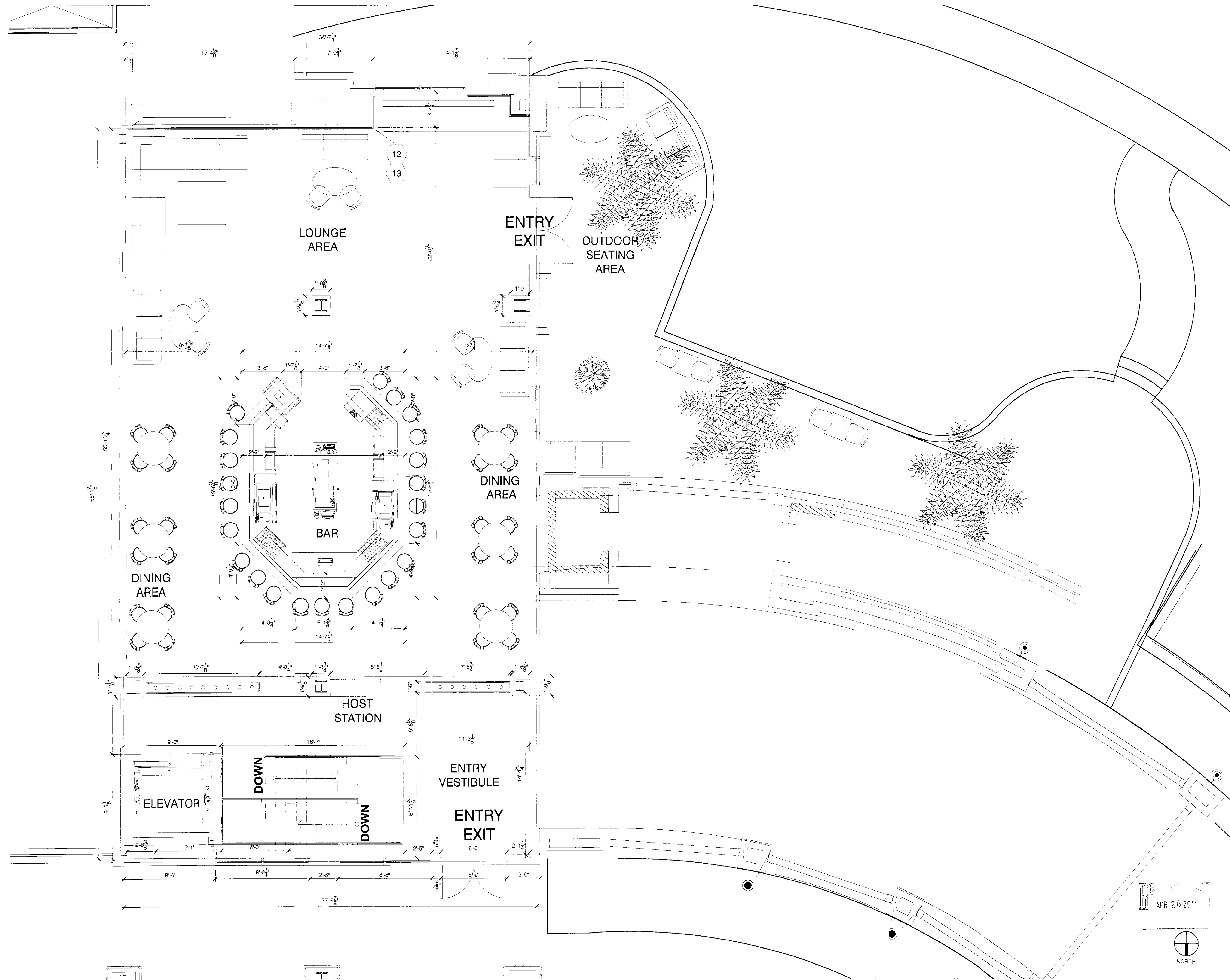
PODIUM LEVEL FLOOR PLAN
