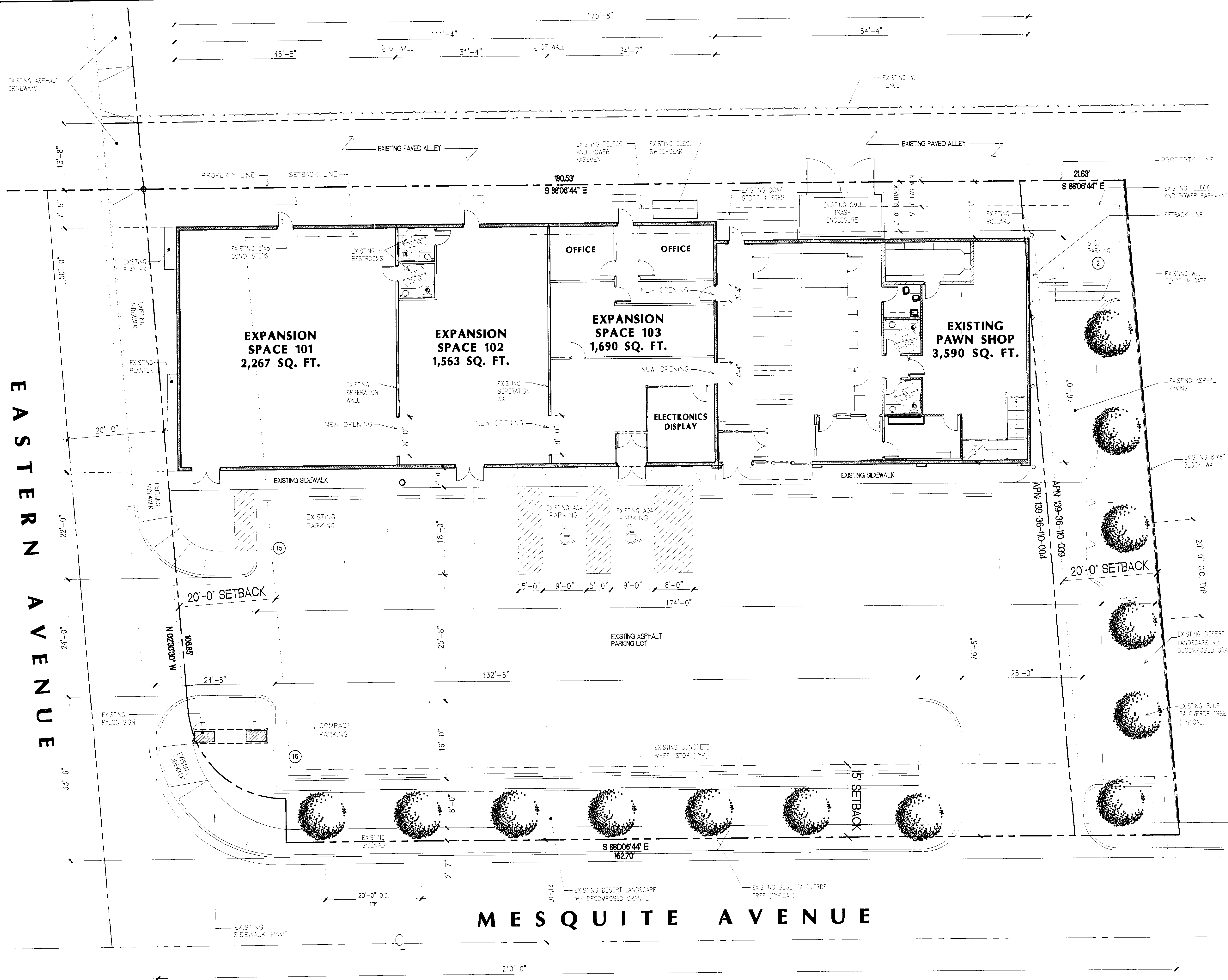
1 SITE PLAN SCALE: 1/4"=1'-0"
