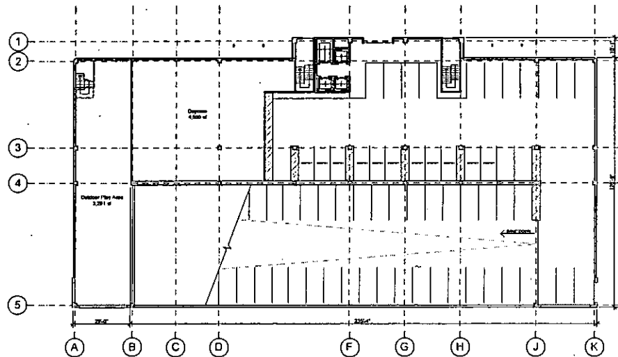
Eighth Floor
