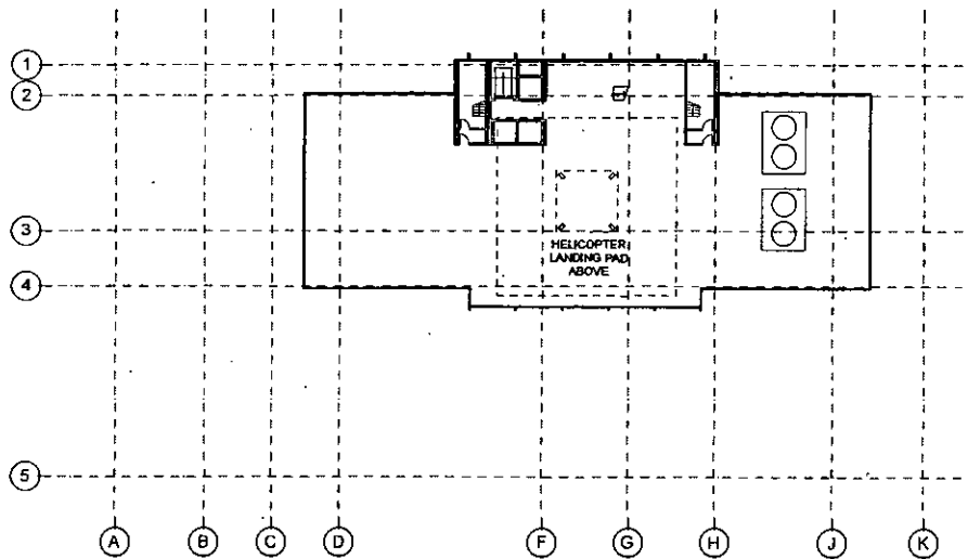
Roof Plan
