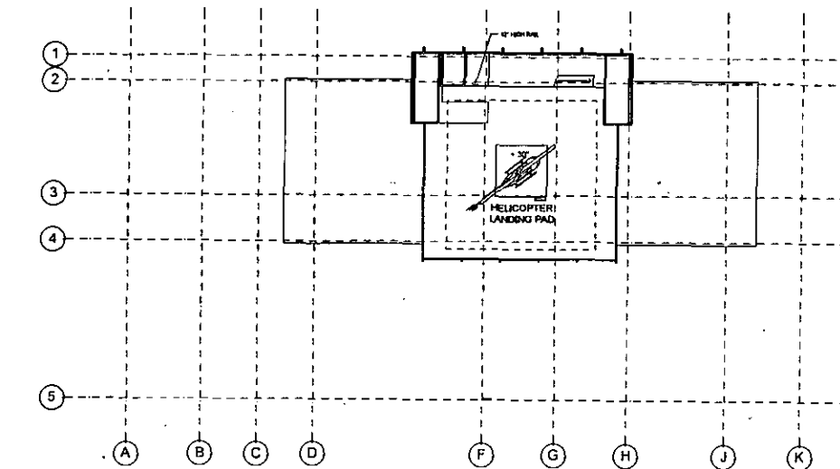
Roof 2 Plan
