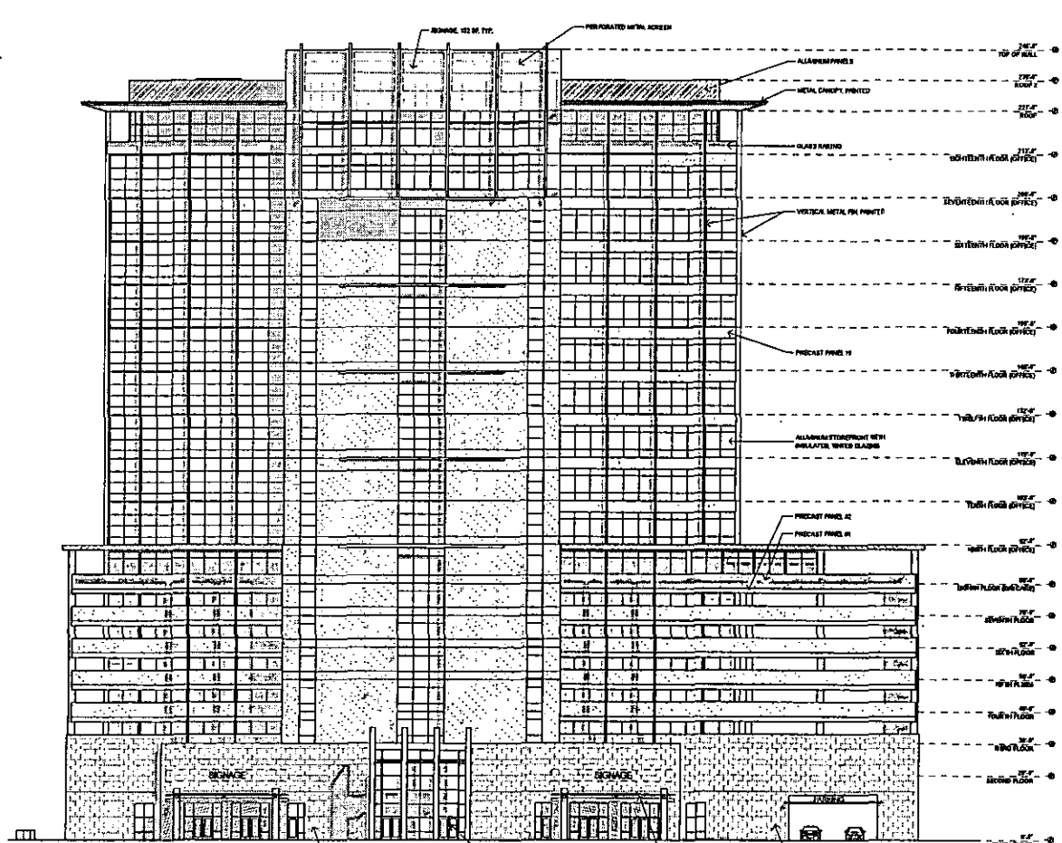
D2 NORTH ELEVATION 1/8" = 1'-0"
