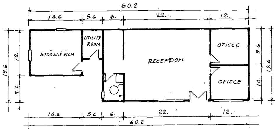
FLOOR PLAN (B) (B)
