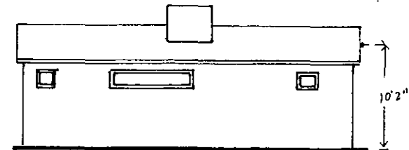
NORTH ELEVATION (C)
