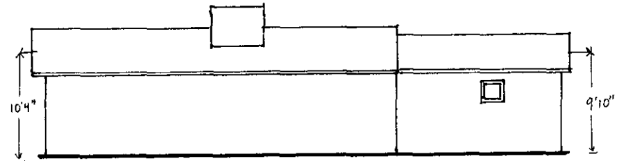
NORTH ELEVATION (B) (B)
