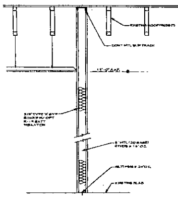
5 INTERIOR WALL DETAIL 1 X R EXISTING WALL
