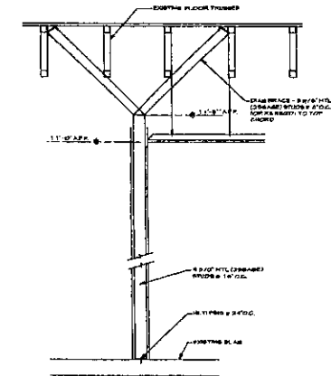
6 INTERIOR WALL DETAIL 1 X R EXISTING WALL
