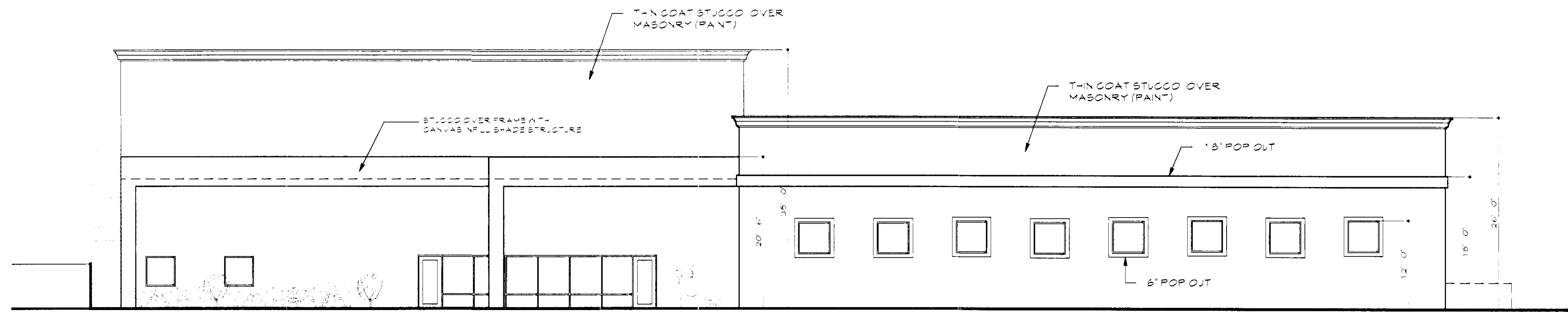
SOUTH ELEVATION
