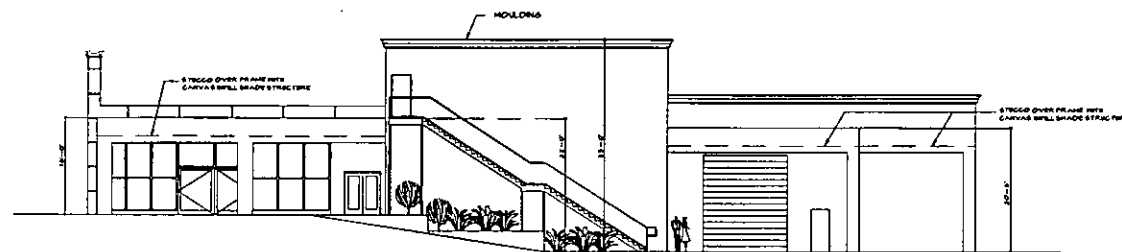
WEST ELEVATION
