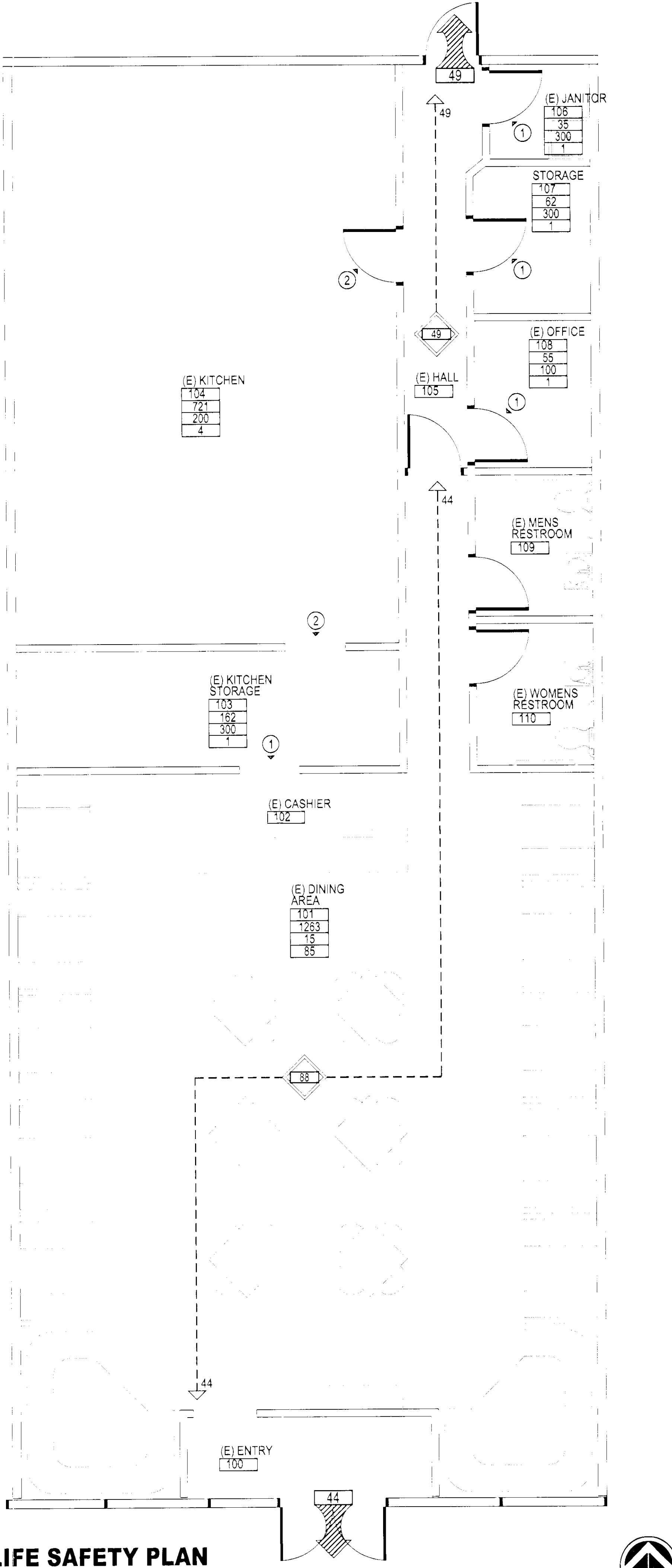
LIFE SAFETY PLAN
