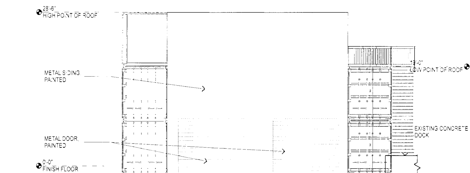
EAST ELEVATION
