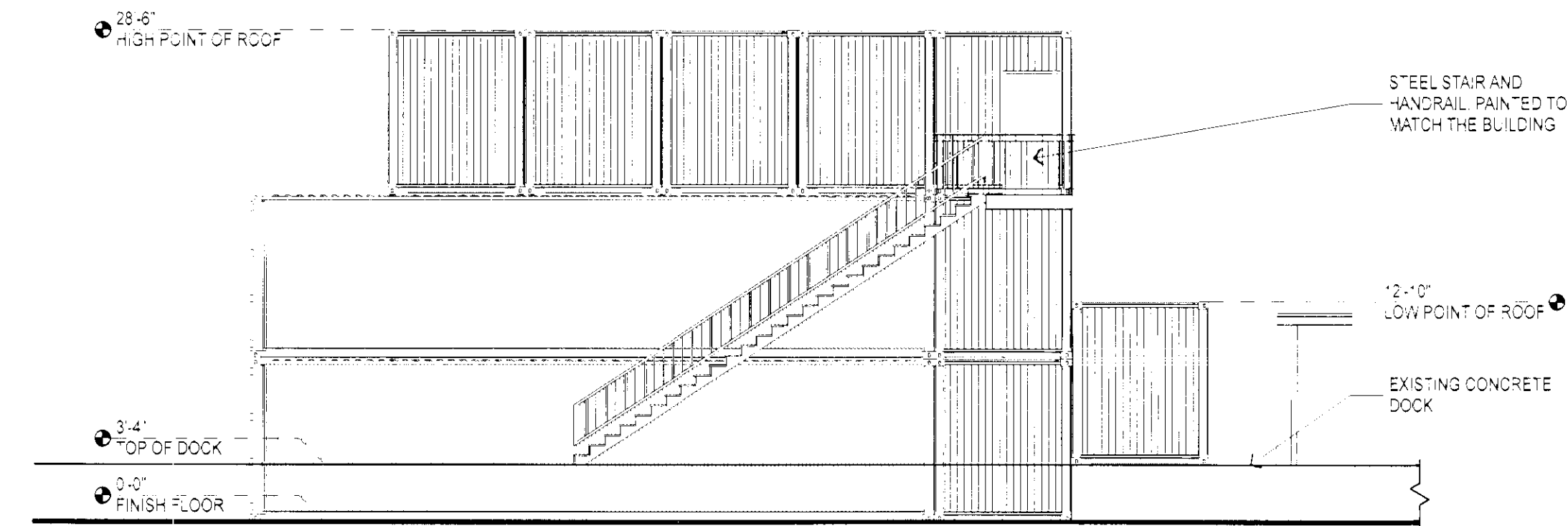
NORTH ELEVATION
