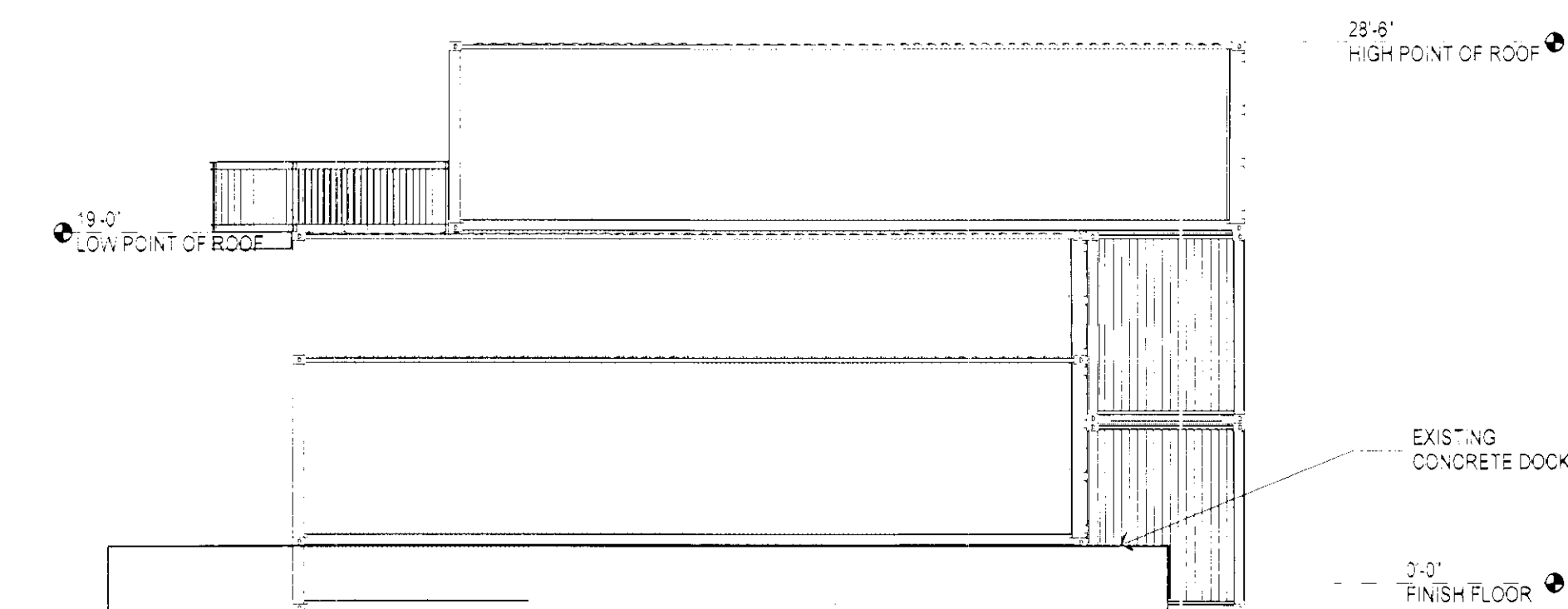
WEST ELEVATION
