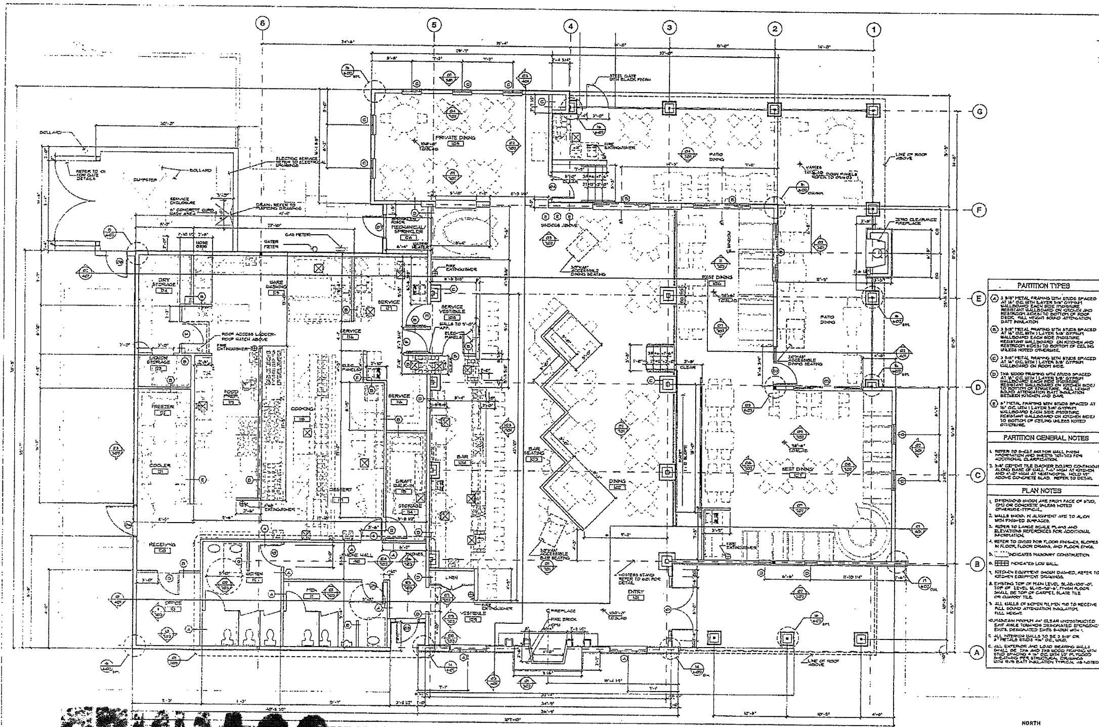
01 FLOOR PLAN 1/4"=1'-0"
