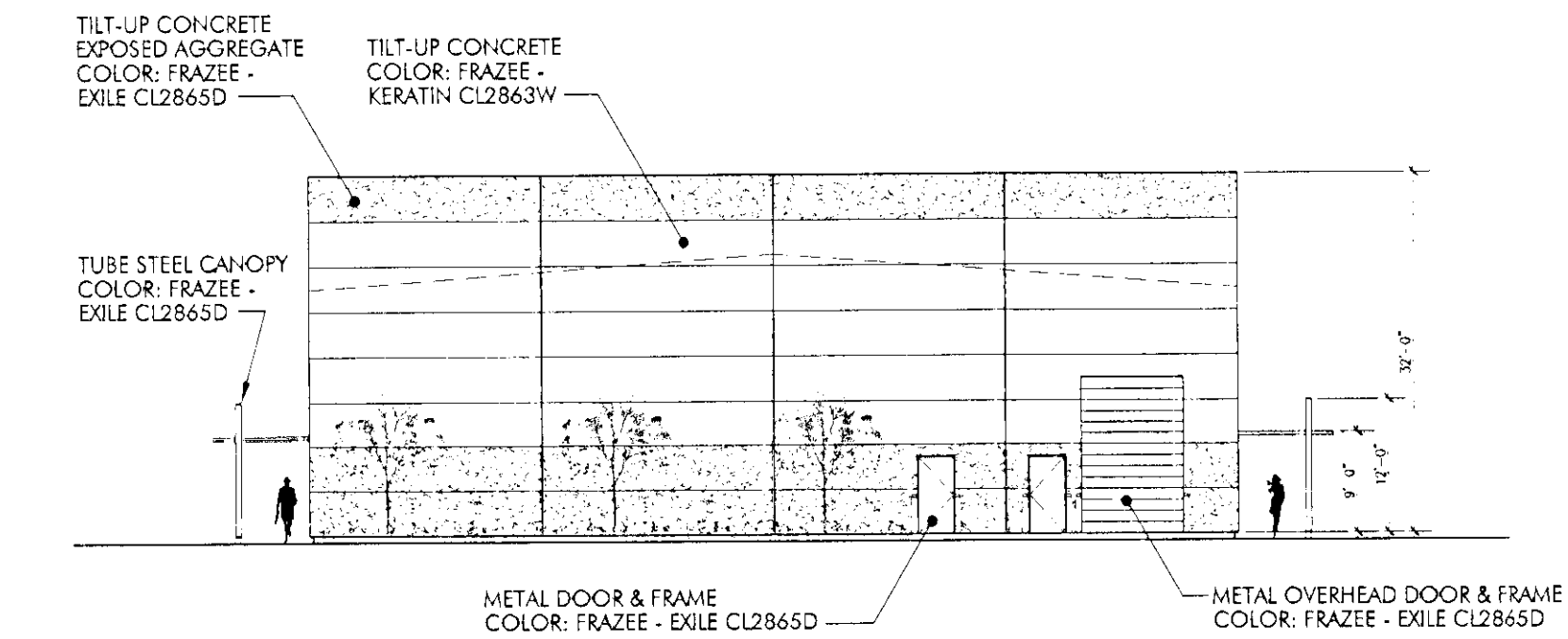
NORTH ELEVATION
