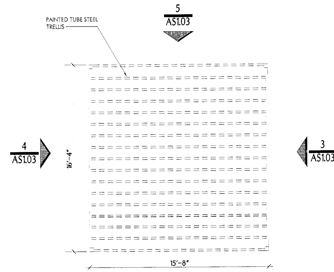
2 TYPICAL TRASH ENCLOSURE PLAN SCALE: 1/4" = 1'-0"
