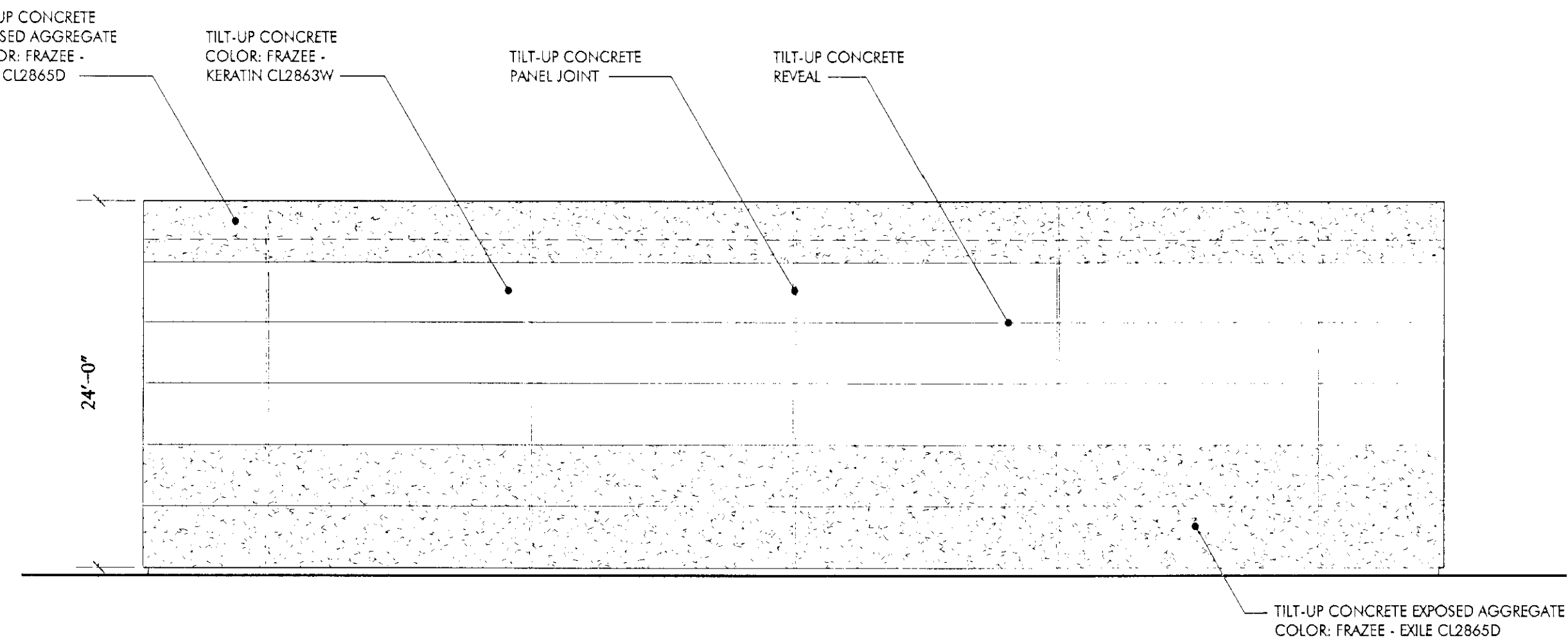
2 BUS WASH SOUTH ELEVATION SCALE: 1/8" = 1'-0"
