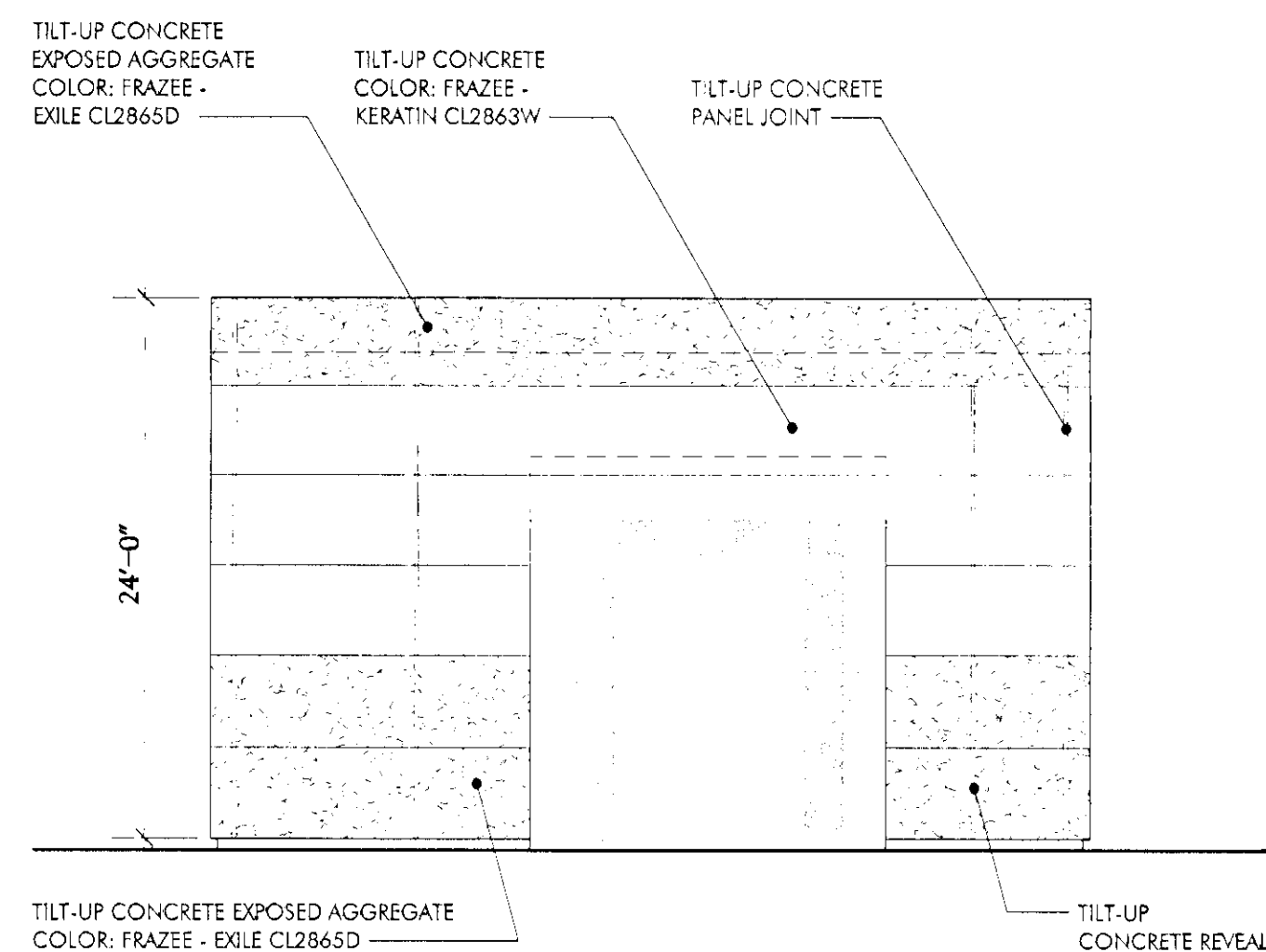
4 BUS WASH WEST ELEVATION SCALE: 1/8" = 1'-0"
