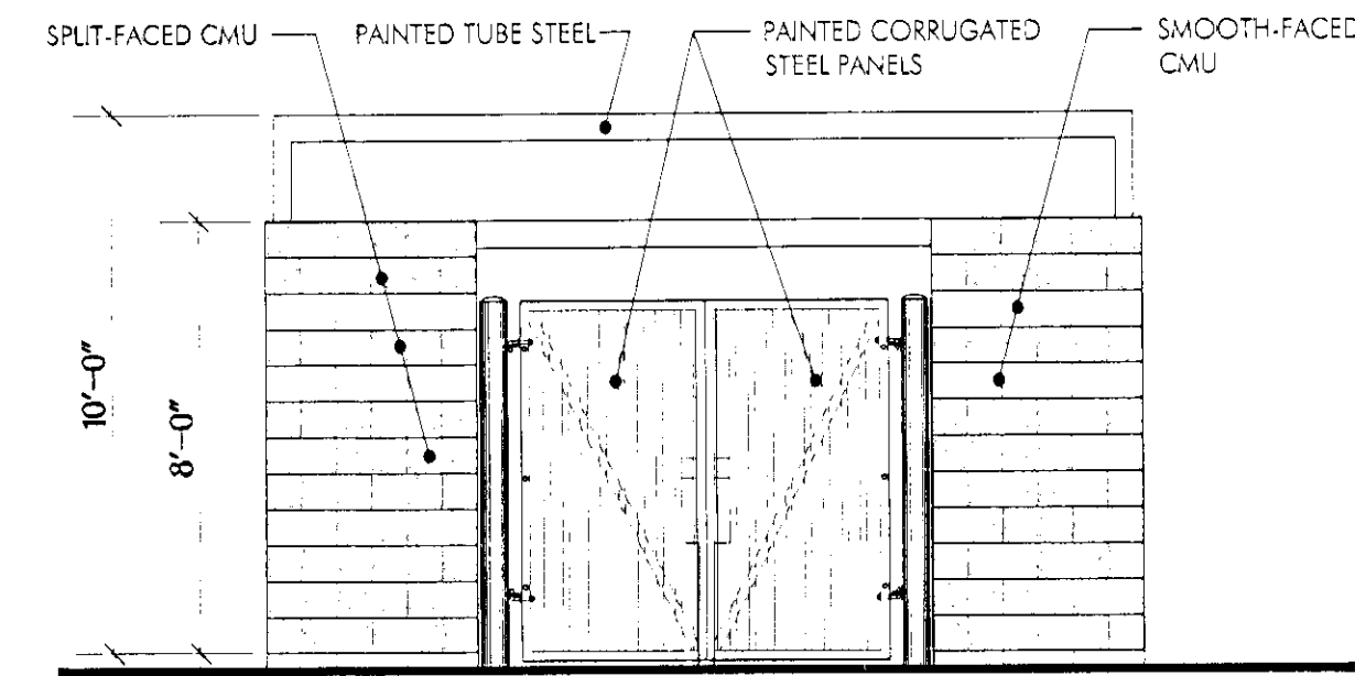
3 TYPICAL TRASH ENCLOSURE ELEVATION SCALE: 1/4" = 1'-0"
