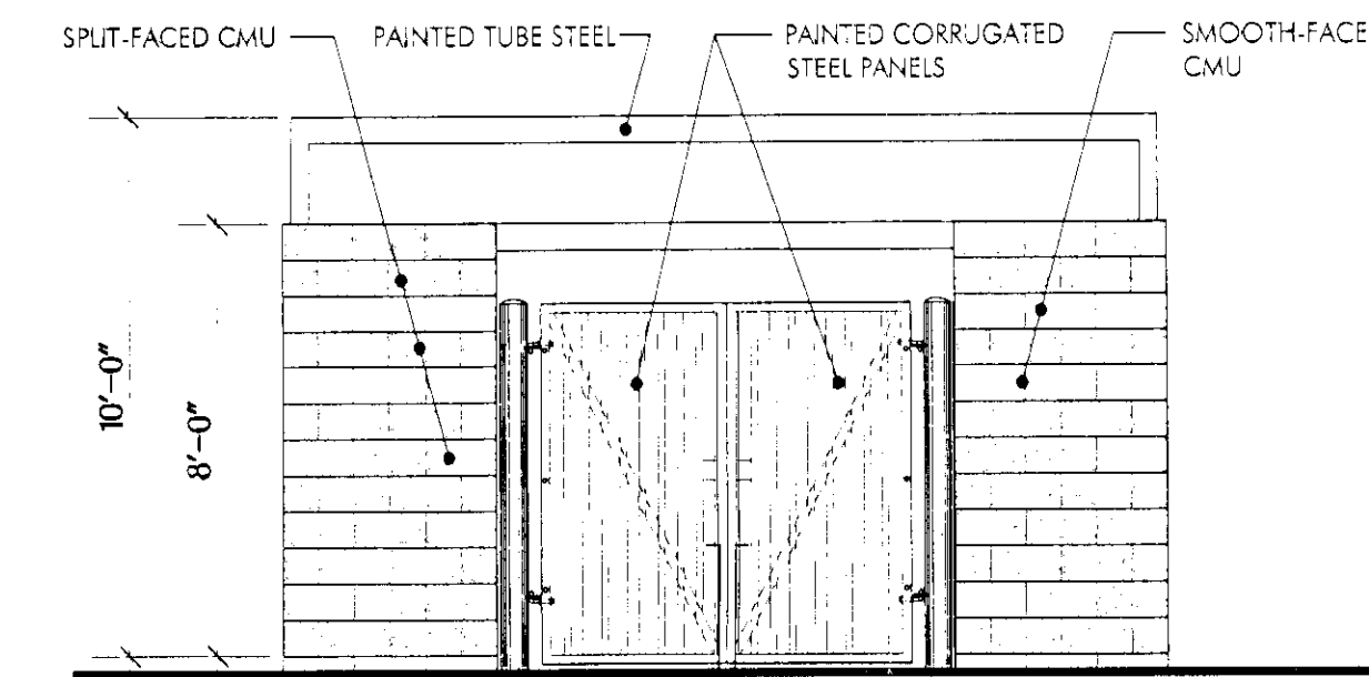
3 SCALE: 1/4" = 1'-0" TYPICAL TRASH ENCLOSURE ELEVATION
