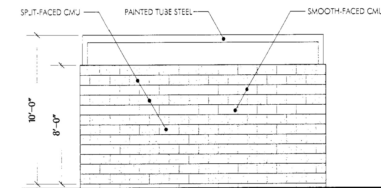
4 SCALE: 1/4" = 1'-0" TYPICAL TRASH ENCLOSURE ELEVATION
