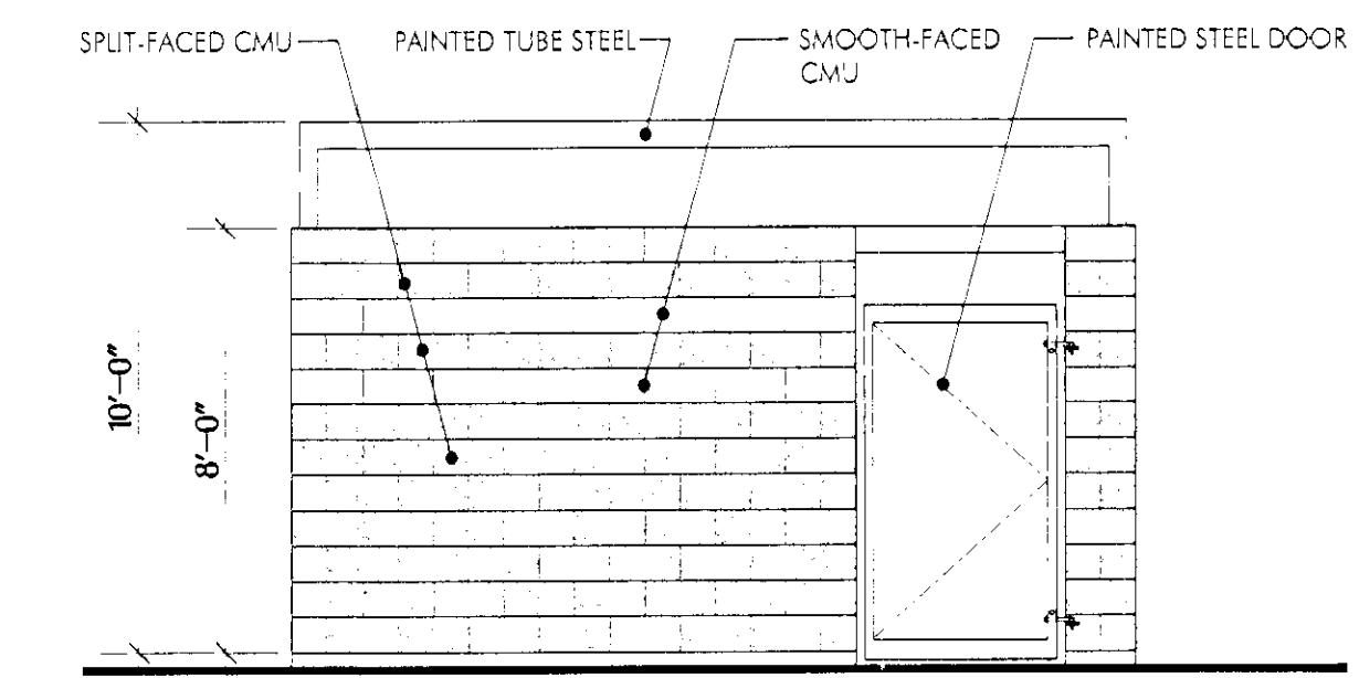
5 TYPICAL TRASH ENCLOSURE ELEVATION SCALE: 1/4" = 1'-0"
