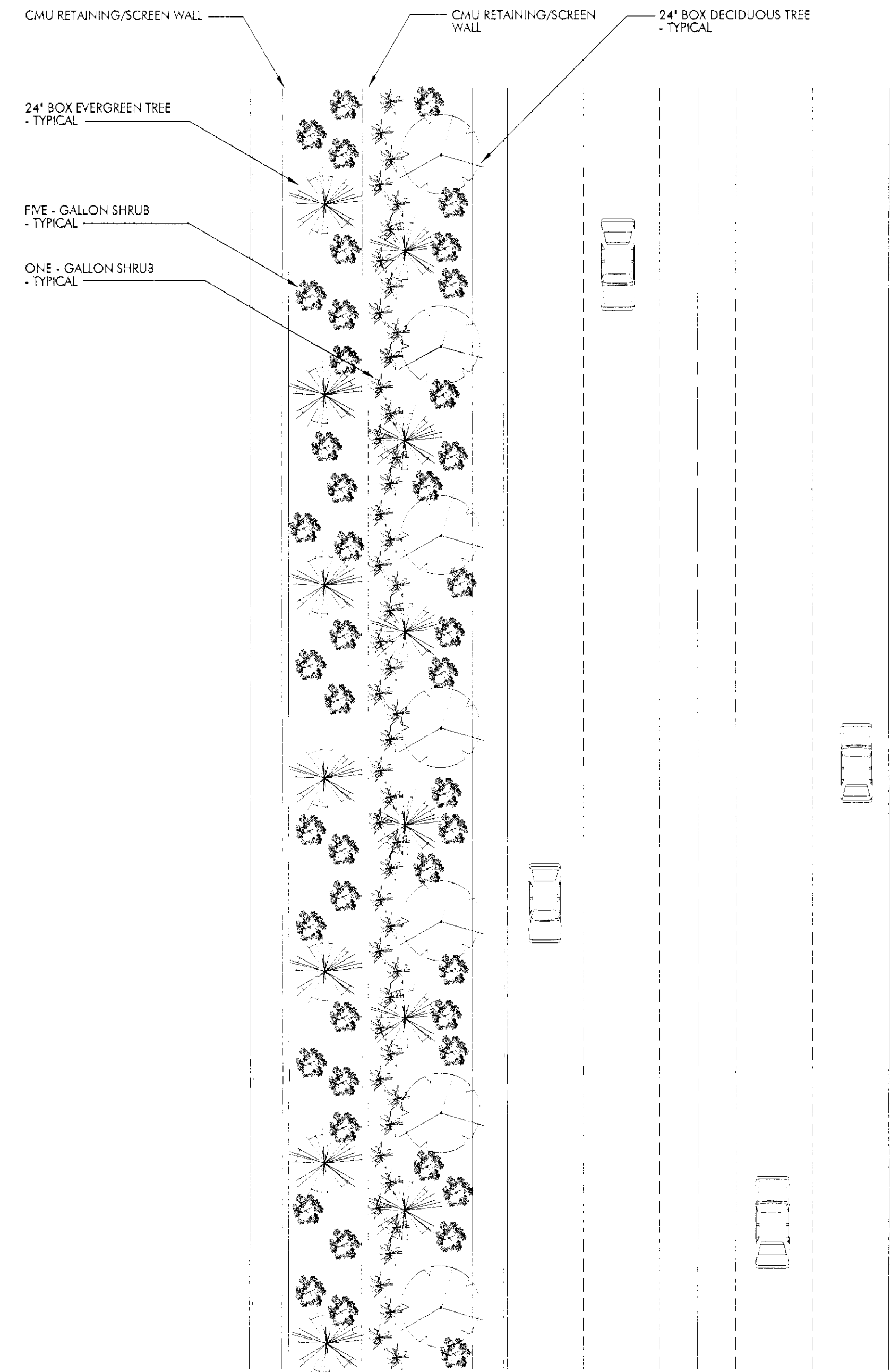
2 LANDSCAPE BUFFER DETAIL SCALE: 1/16" = 1'-0"
