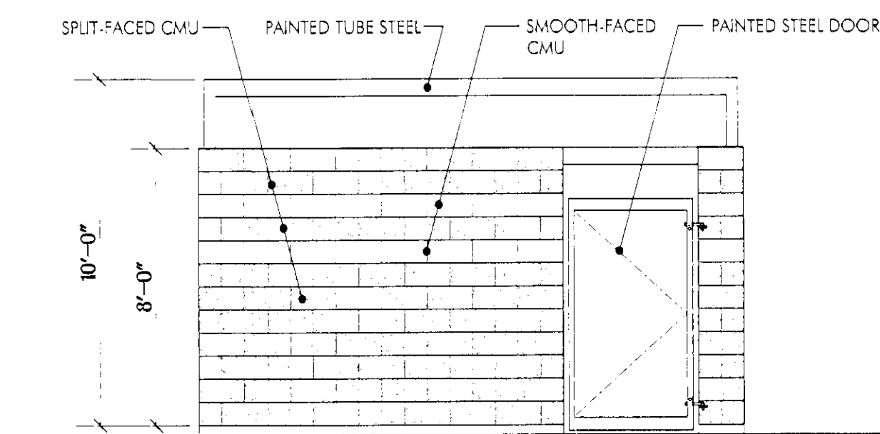
5 SCALE: 1/4" = 1'-0" TYPICAL TRASH ENCLOSURE ELEVATION
