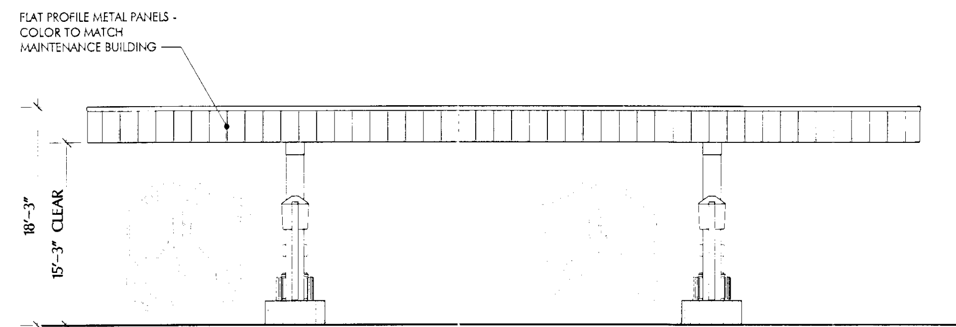
5 BUS FUELING STATION ELEVATION SCALE: 1/8" = 1'-0"
