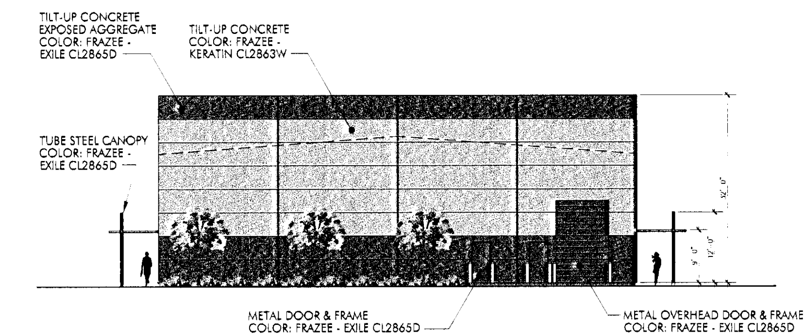
NORTH ELEVATION
