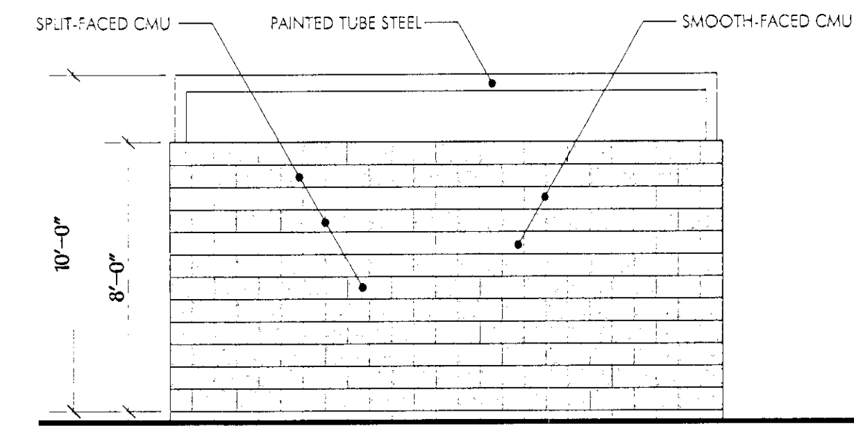
4 TYPICAL TRASH ENCLOSURE ELEVATION SCALE: 1/4" = 1'-0"
