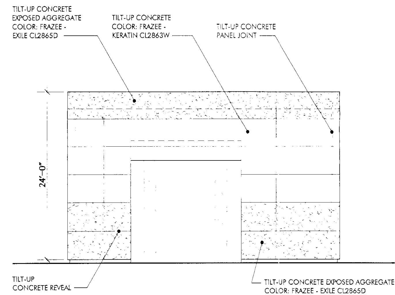
3 BUS WASH EAST ELEVATION SCALE: 1/8" = 1'-0"
