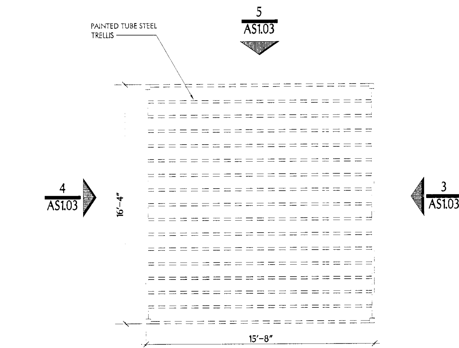
2 SCALE: 1/4" = 1'-0" TYPICAL TRASH ENCLOSURE PLAN
