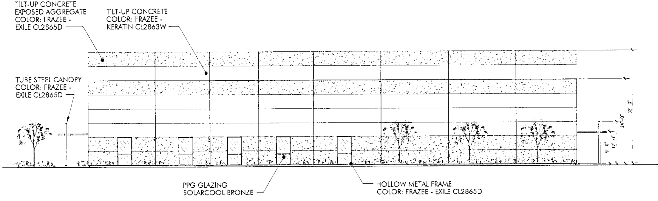
SOUTH ELEVATION
