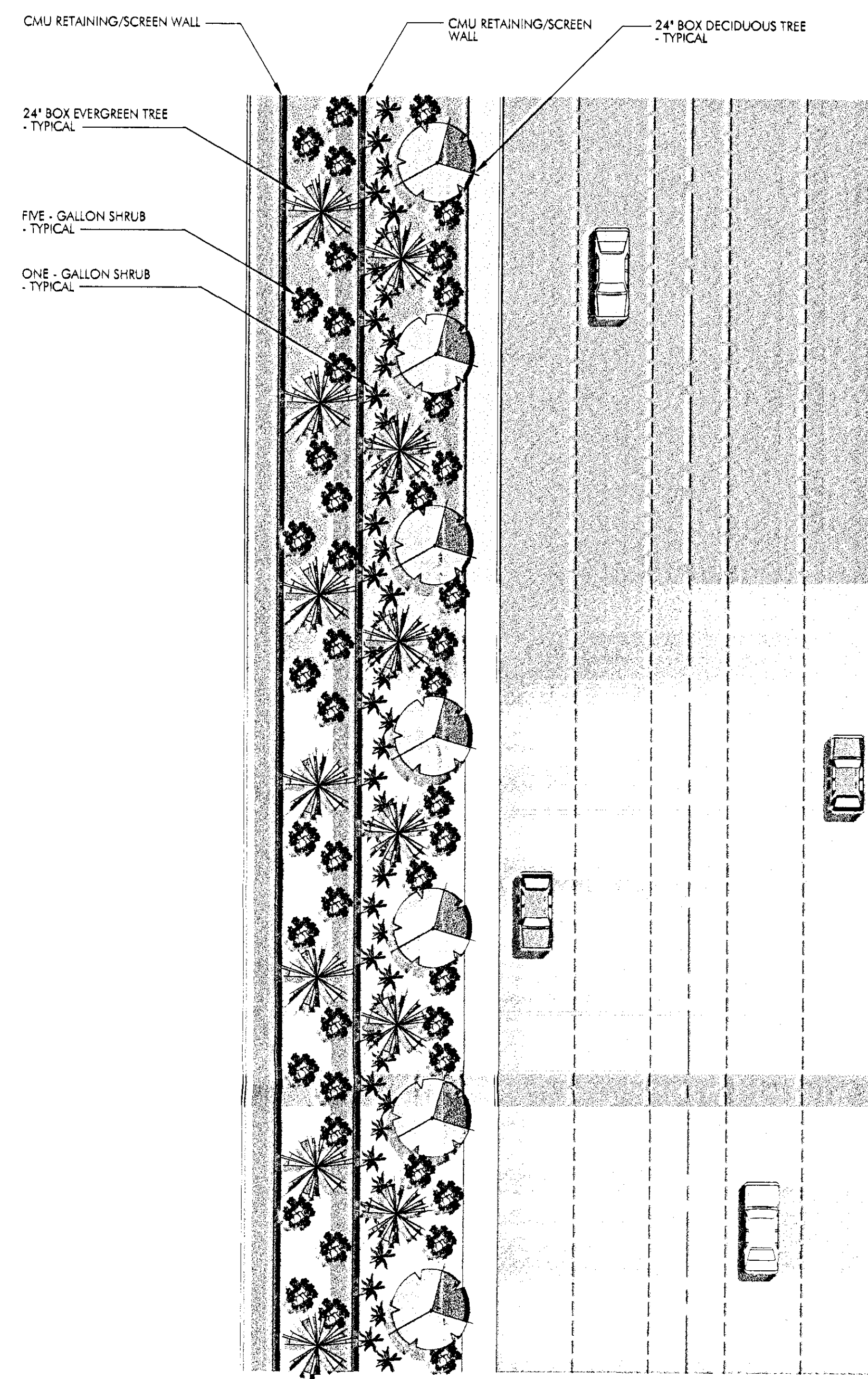
2 LANDSCAPE BUFFER DETAIL SCALE: 1/16" = 1'-0"
