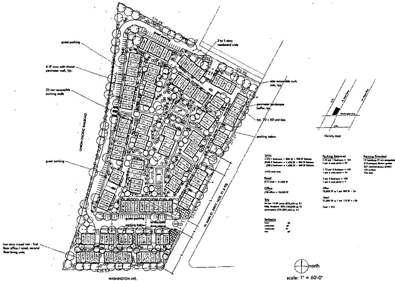
Site/Landscape Plan
