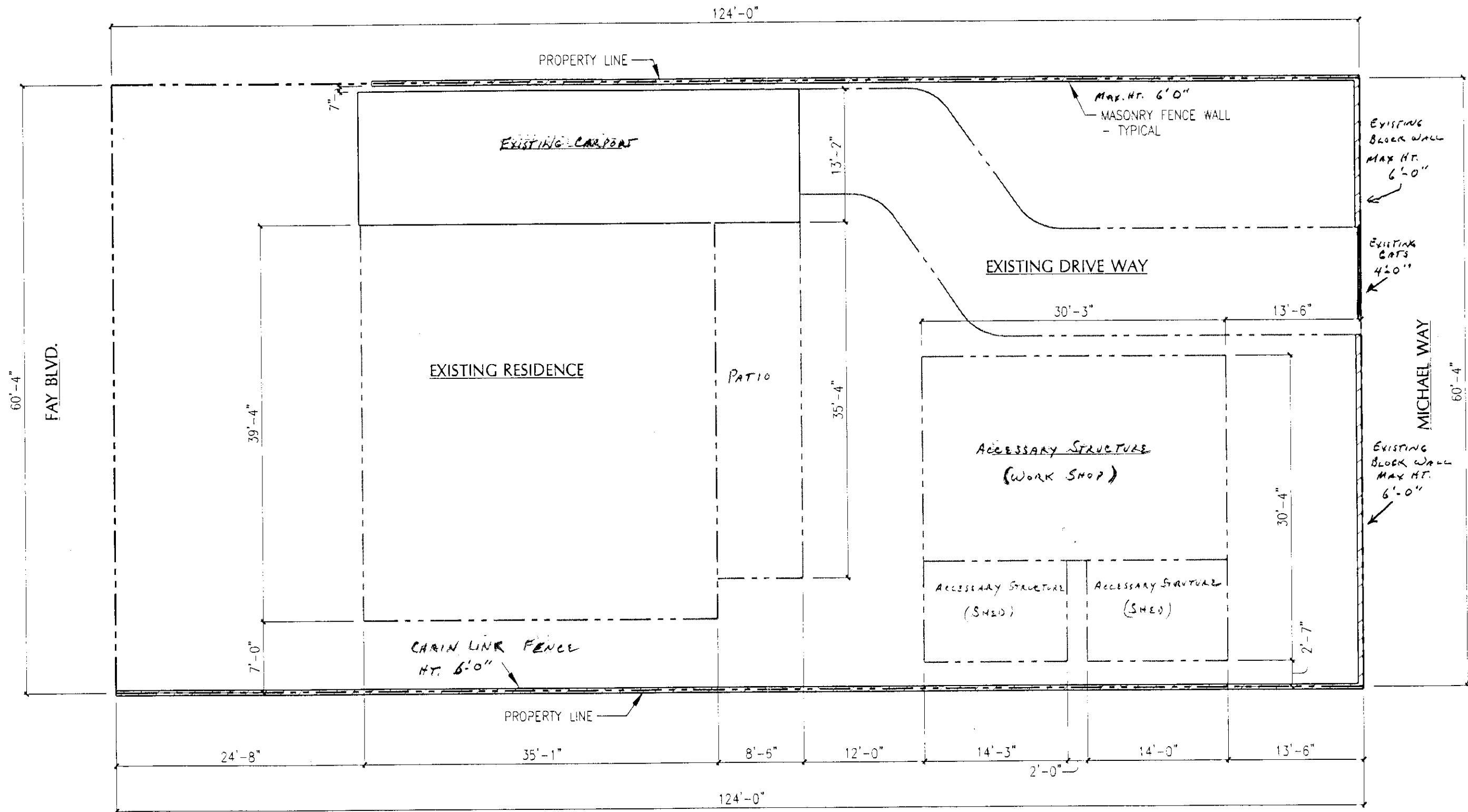
FOUNDATION PLAN
