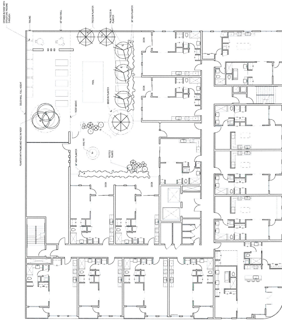
FIFTH FLOOR 1/8" = 1'-0"
