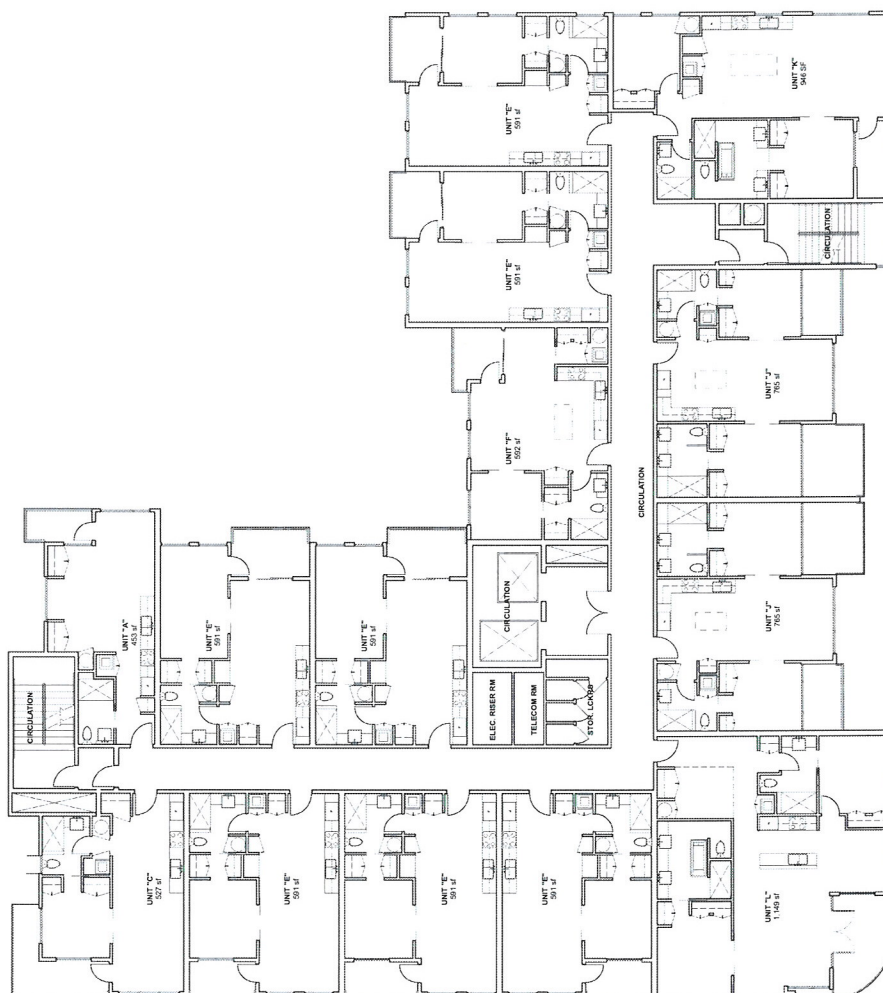
EIGHTH FLOOR 1/8" = 1'-0"
