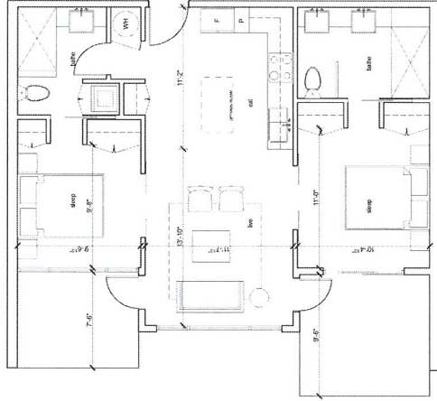
TYPICAL 2-BEDROOM
