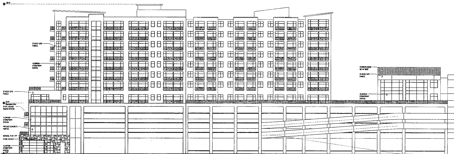
EAST ELEVATION
