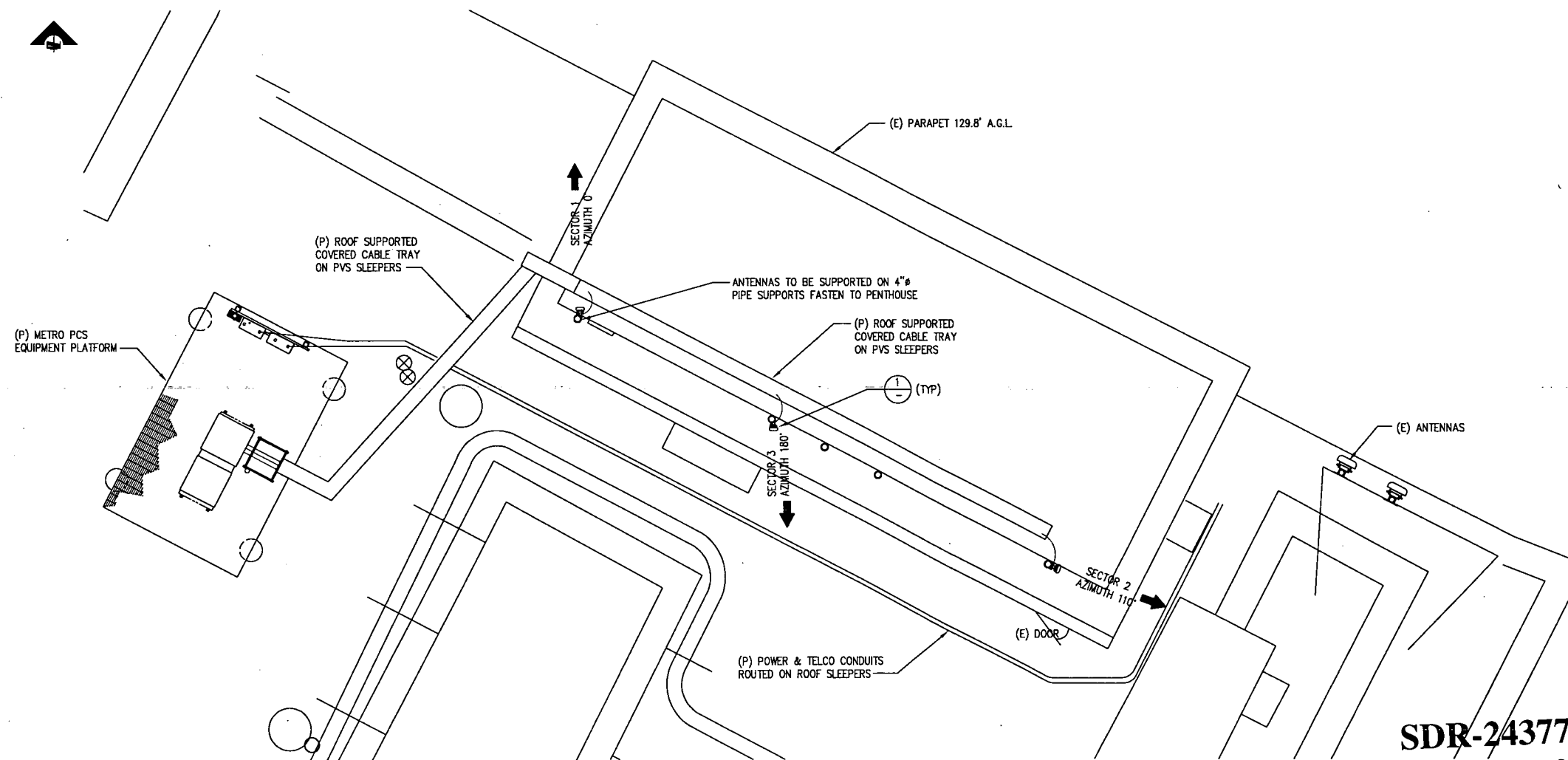
ANTENNA DETAILS
