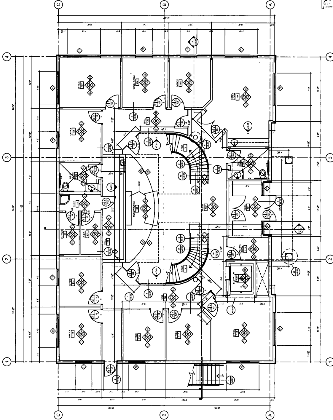
1 MAIN LEVEL FLOOR PLAN SCALE: 1/4" = 1'-0"
