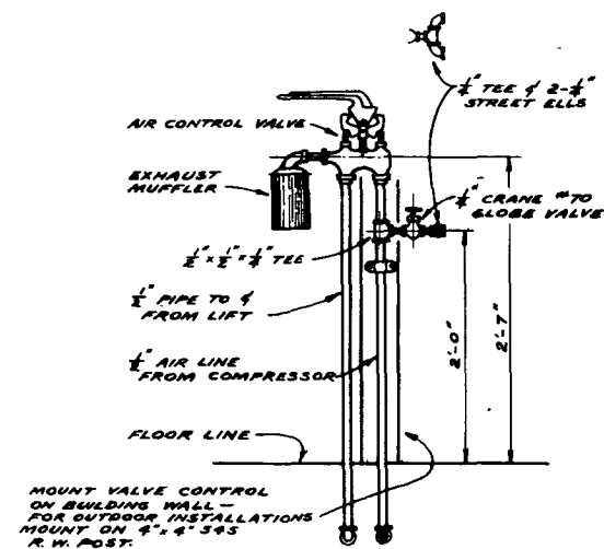
DETAIL OF LIFT CONTROL
