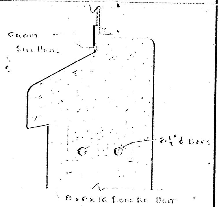
ALTERNATE 5 FOR SILL ⑭
