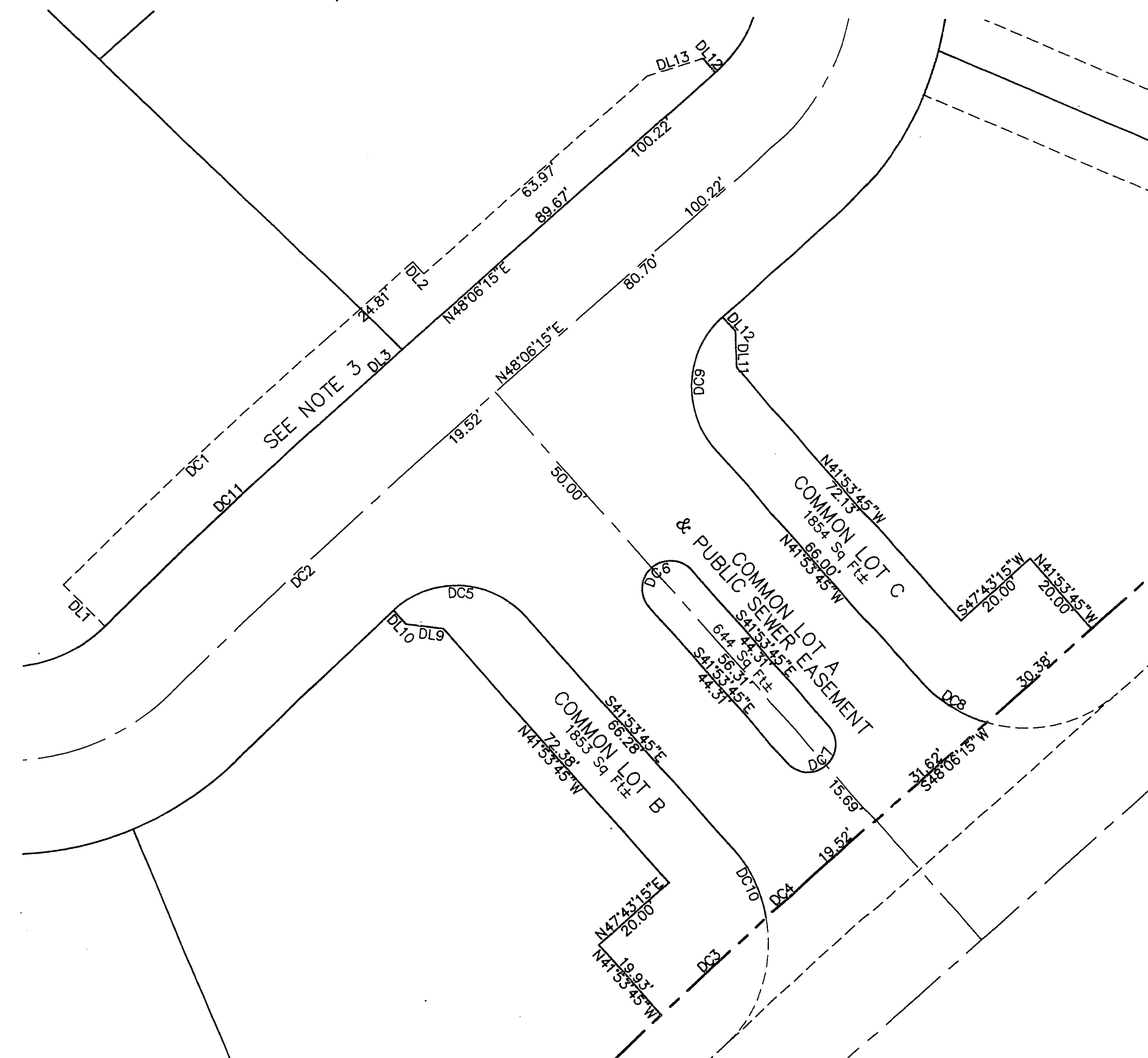
DETAIL 3 SCALE: 1"=20'
