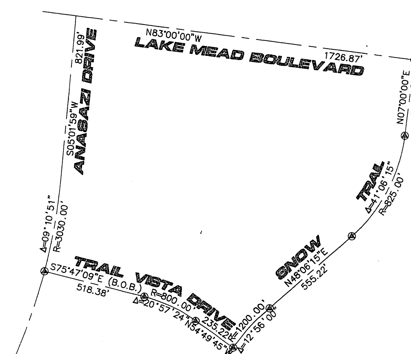
SURVEY ANALYSIS
