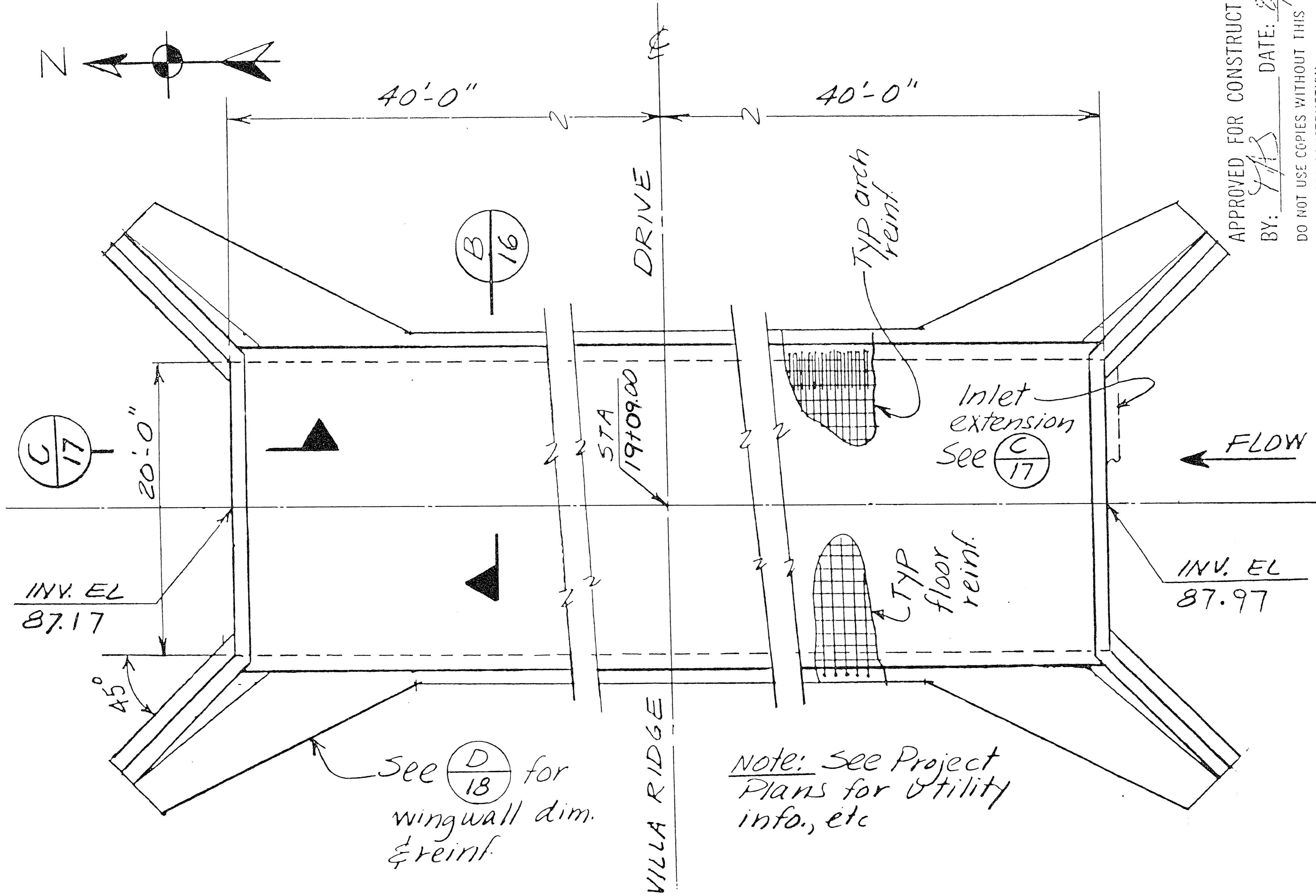
PLAN - ARCH CULVERT @ STA 19 + 09.00 VILLA RIDGE DRIVE Scale 1" = 10'-0" A
