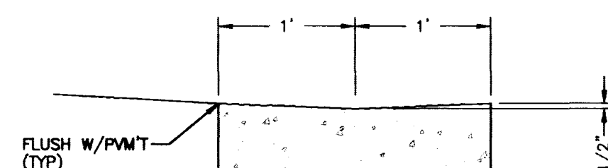
DETAIL "G" NTS
