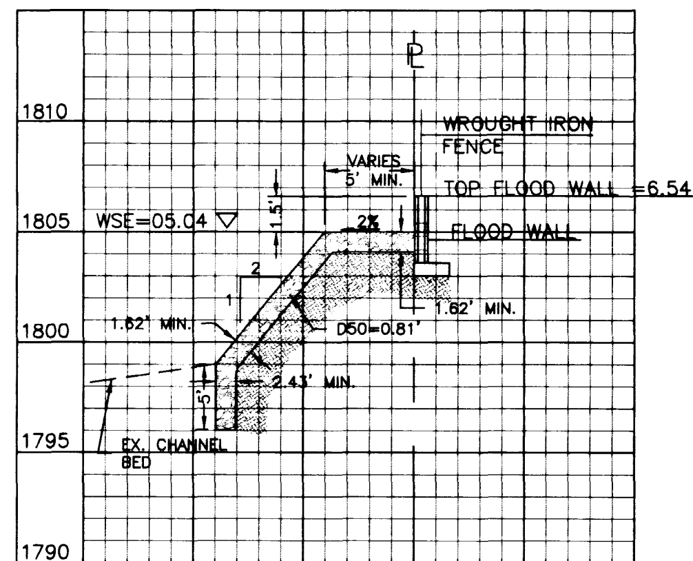
SECTION D1 - D1 STA=9+00 NORTH PROPERTY LINE Q=12,000 NTS
