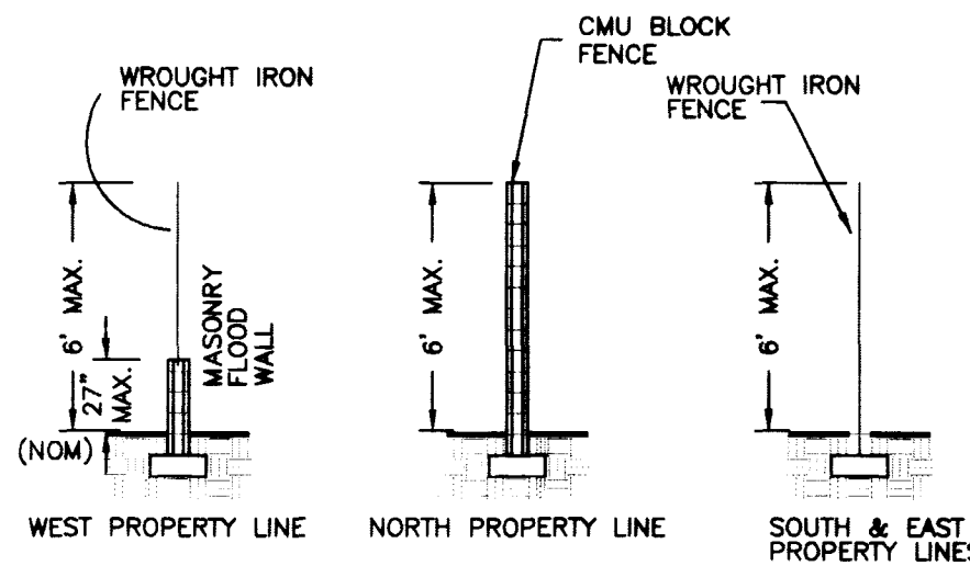
TYPICAL WALL DETAILS NTS
