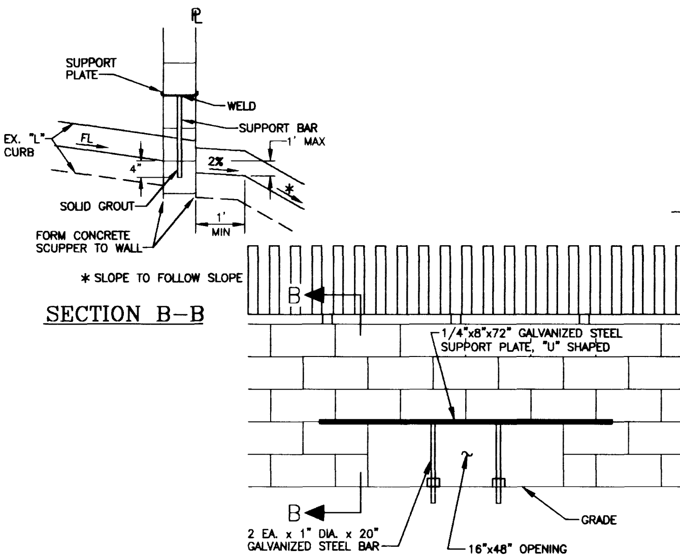
DETAIL "K" NTS
