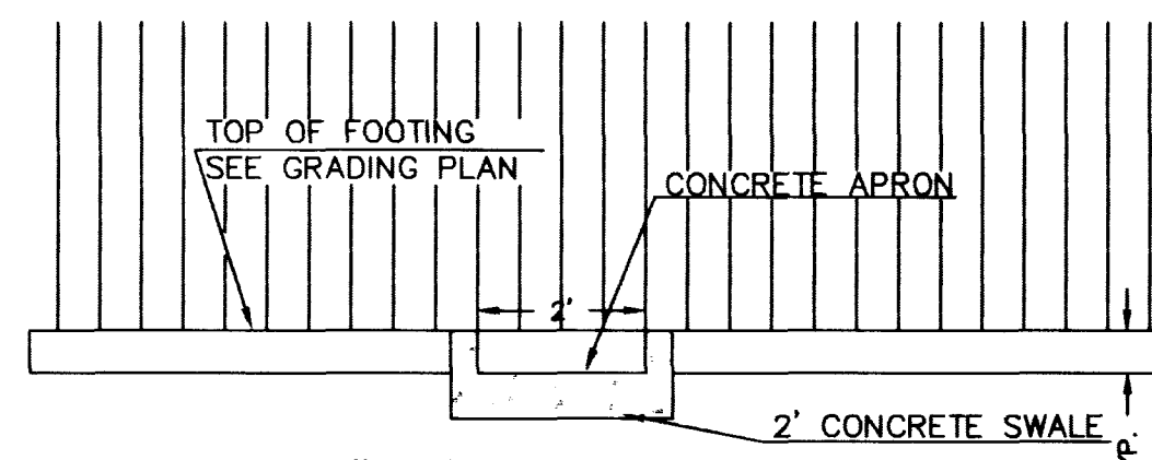
24"x6" OPENING IN WROUGHT IRON FENCE NTS
