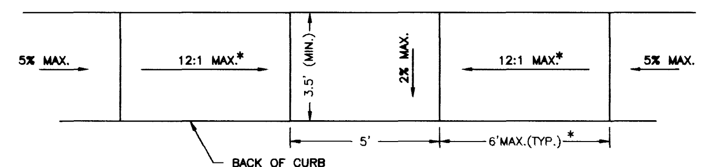
ALT 2 PEDESTRIAN ACCESS RAMP DETAIL "D" NTS
