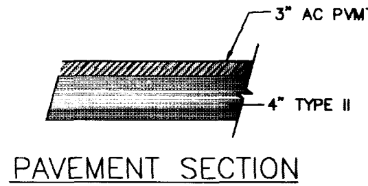
DETAIL "J" NTS
