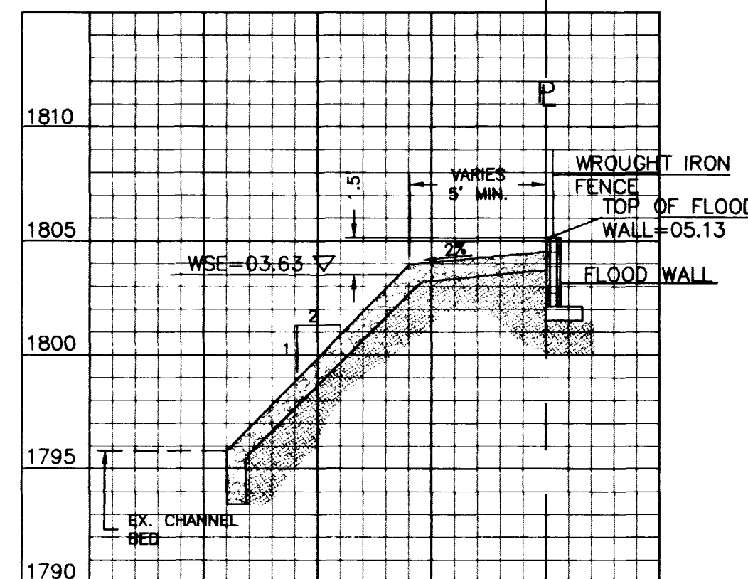
SECTION D3 - D3 STA=4+25(S) PROP LINE Q=12,000 NTS
