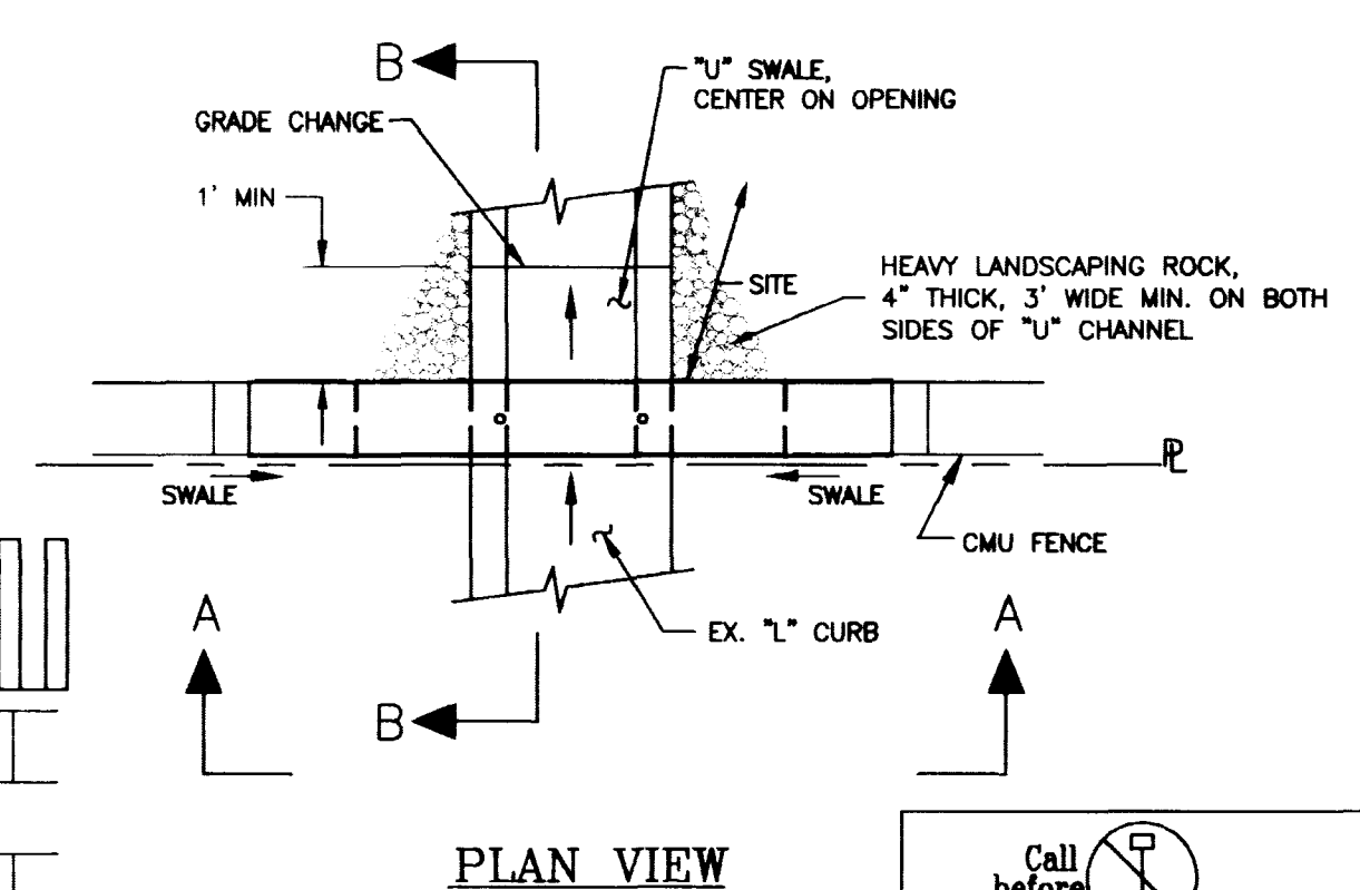
ALT 2 PEDESTRIAN ACCESS RAMP DETAIL "D" NTS
