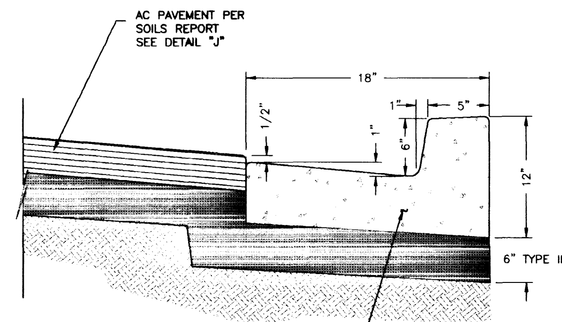
18" "L" CURB DETAIL "A" NTS
