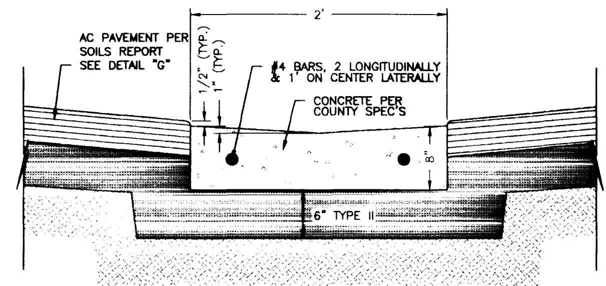
2' VALLEY GUTTER DETAIL "B" NTS
