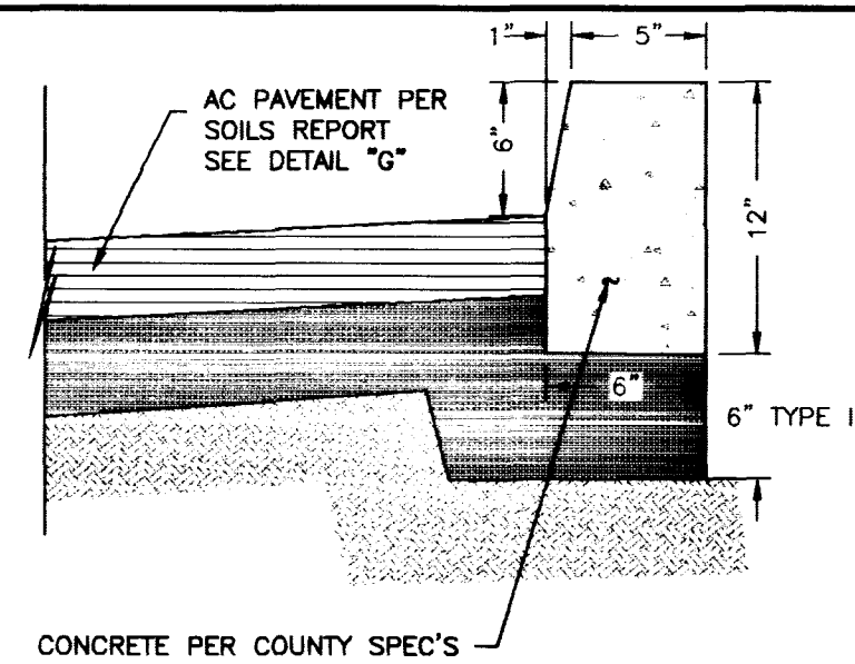
"A" CURB DETAIL "F" NTS
