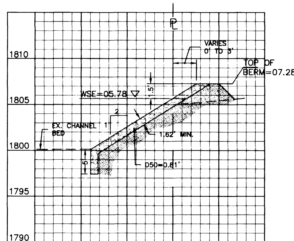
SECTION D2 - D2 STA=10+75 EX. BRIDGE EXTENSION, Q=12,000 NTS
