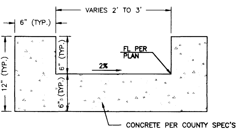
"U" GUTTER DETAIL "C" NTS
