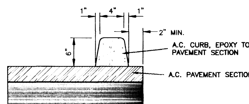
DETAIL "L" NTS
