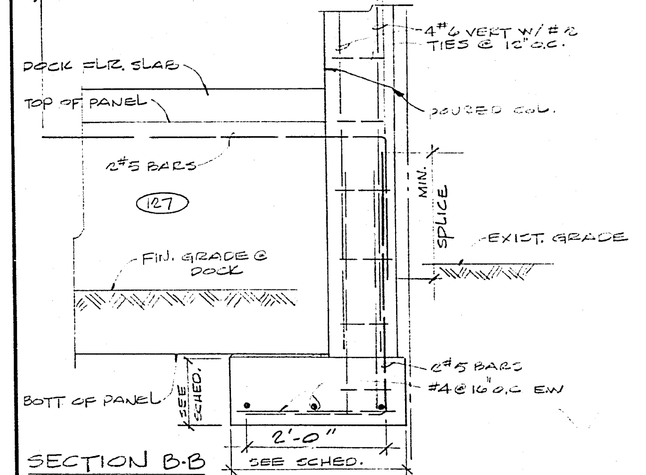
1 PROPERTY LINE FOOTING @ COL. LINE H-3 @ SCALE 3/4"=1'-0"
