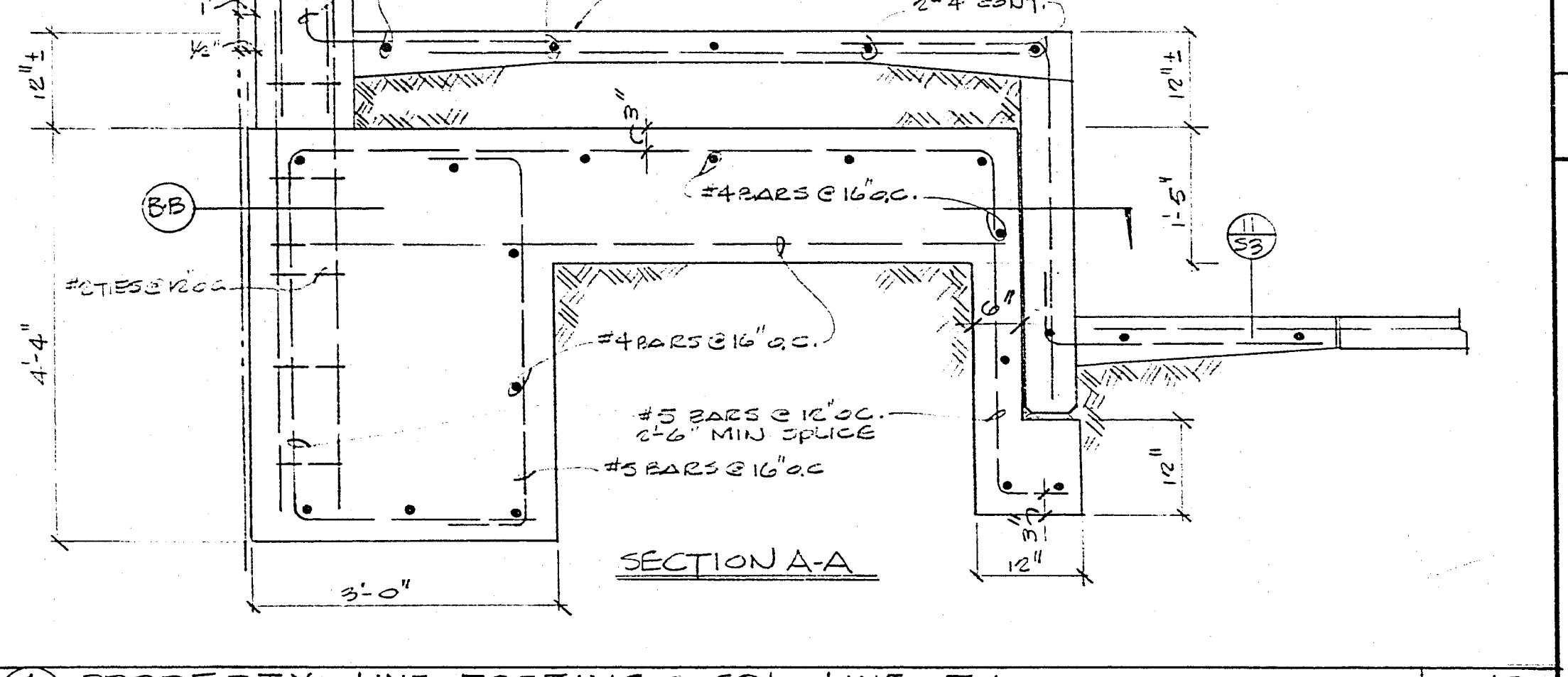
4 PROPERTY LINE FOOTING @ COL. LINE F-1 @ SCALE 3/4"=1'-0"
