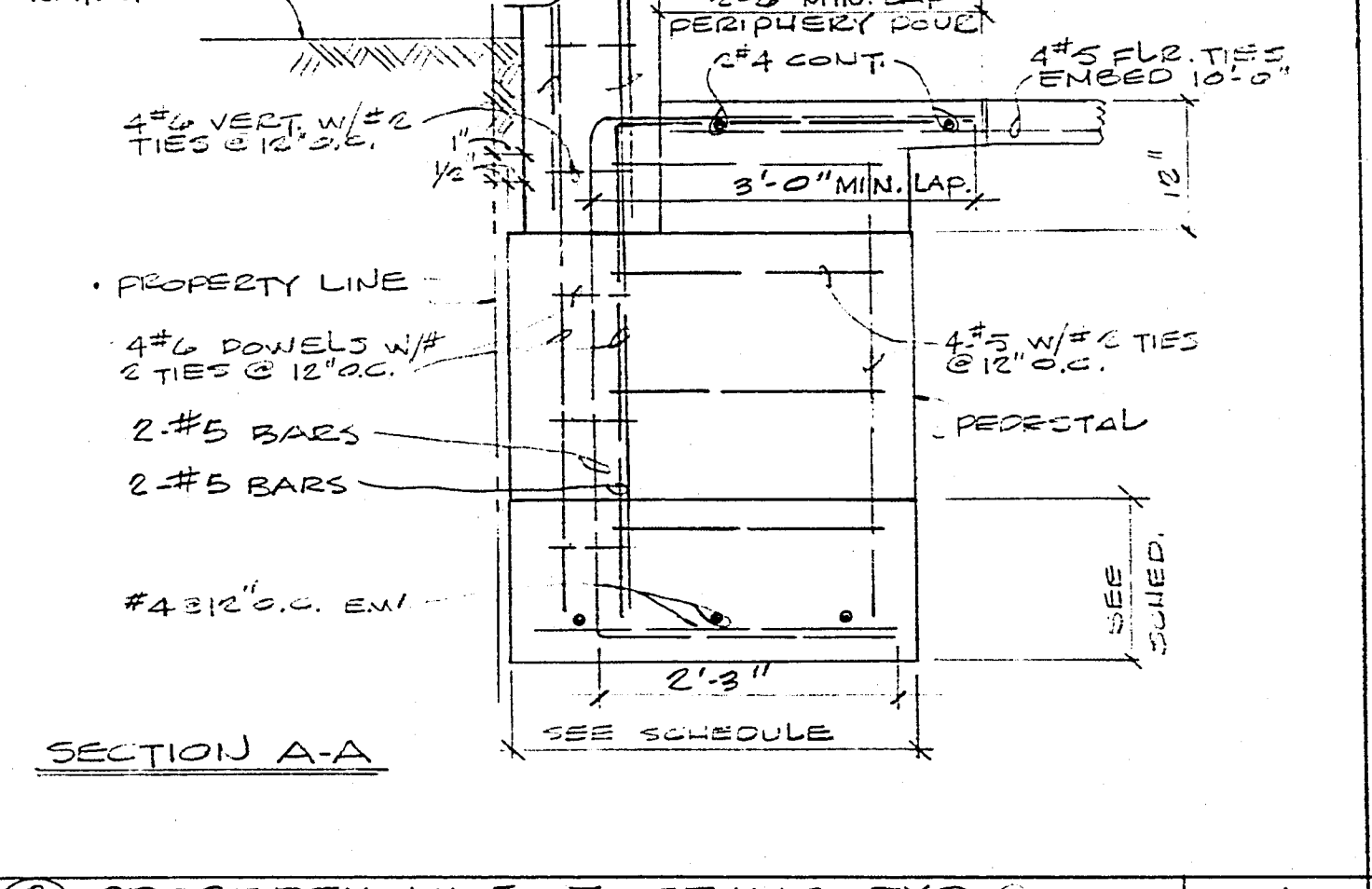
3 PROPERTY LINE FOOTING TYP. @ COL. LINE F-1 @ SCALE 3/4"=1'-0"
