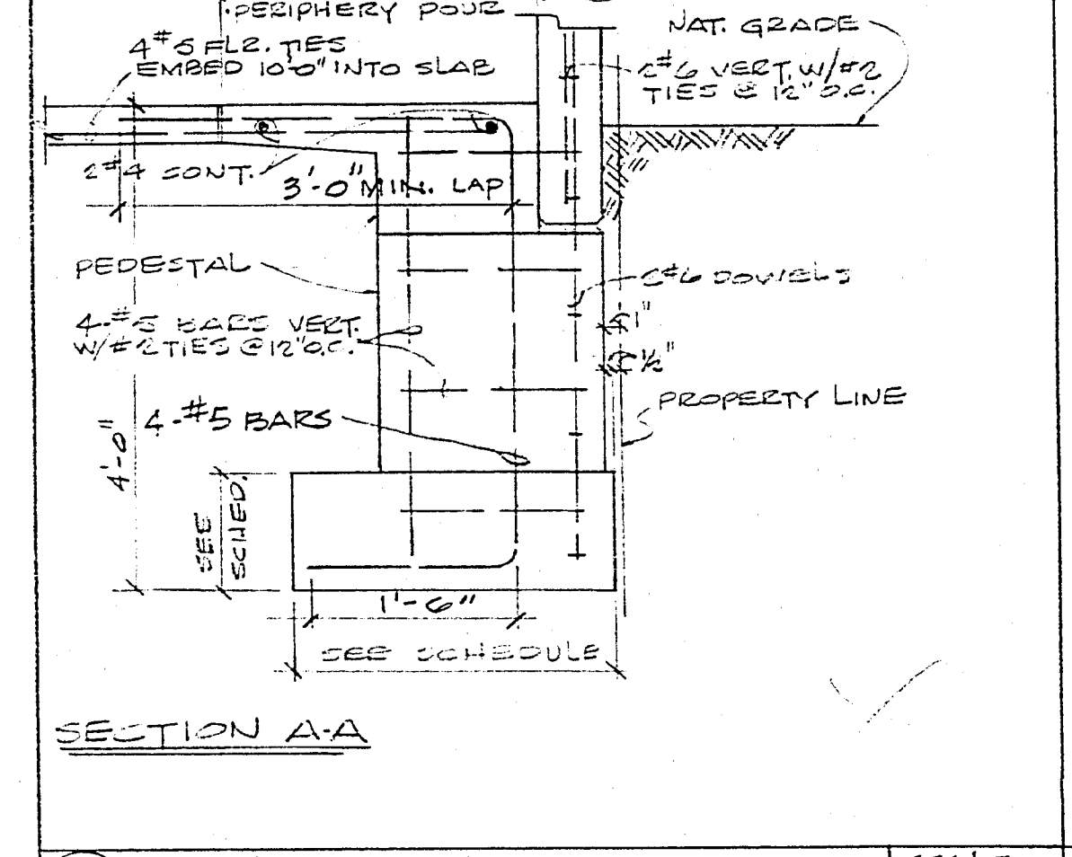
2 PROPERTY LINE FOOTING @ COL. LINE H-1 @ SCALE 3/4"=1'-0"
