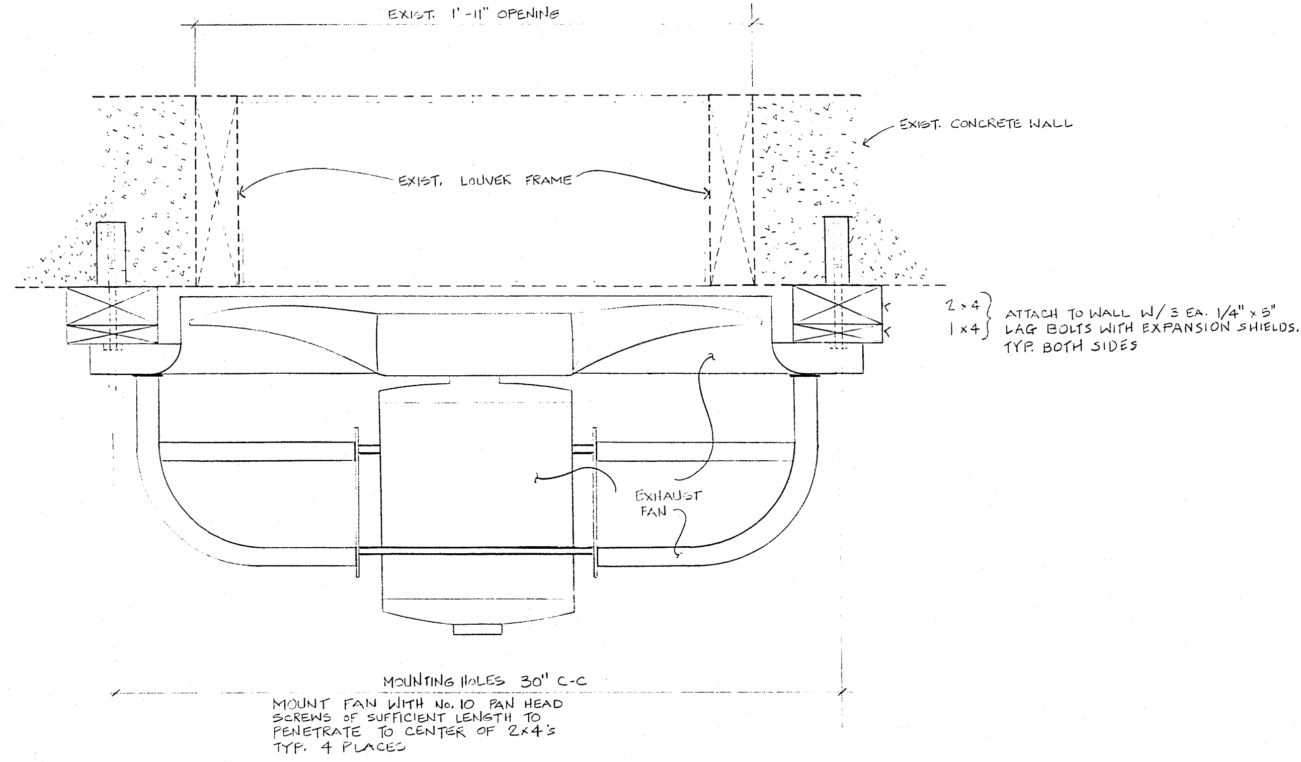
ATTIC EXHAUST FAN MOUNTING DETAIL 2 X-SECTION VIEW FROM TOP SCALE: 3" = 1'-0" M-3
