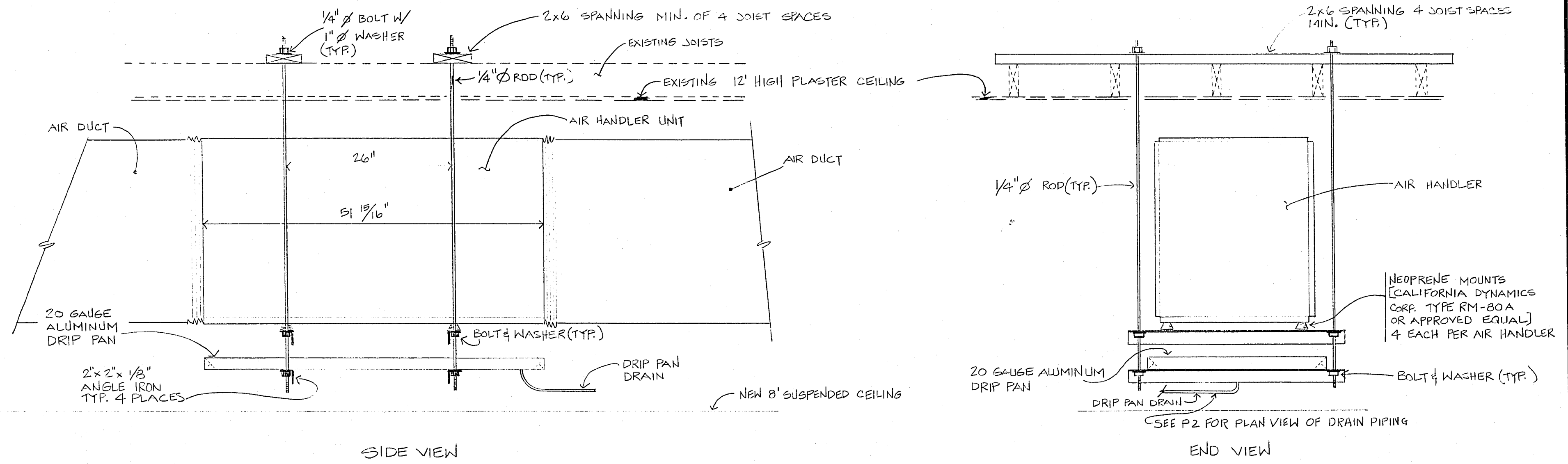
MOUNTING DETAIL FOR AIR HANDLER UNITS 3 SCALE: 1" = 1'-0" M-3
