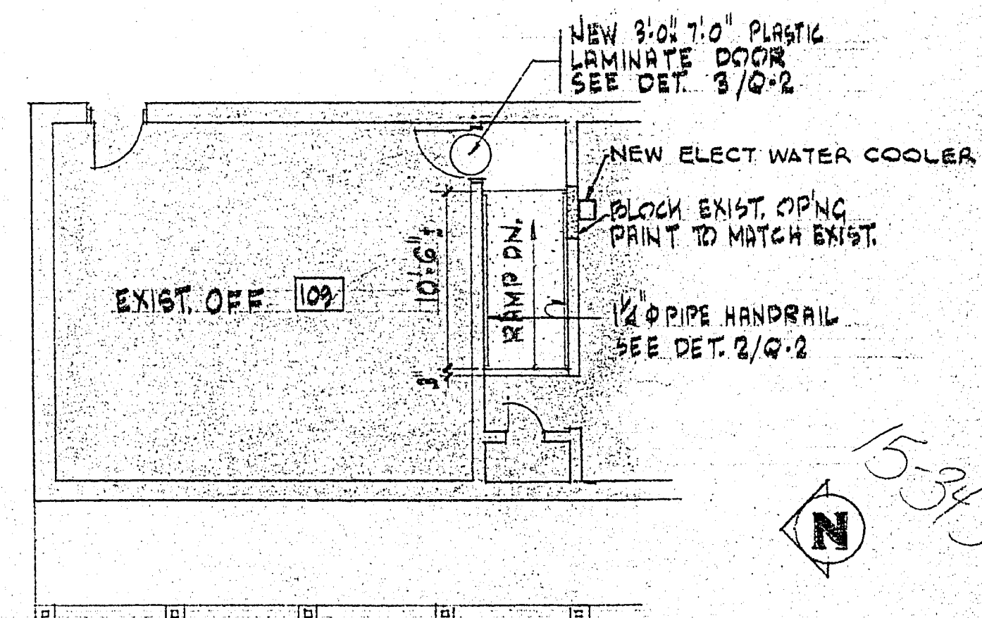
4 PARTIAL FLOOR PLAN Q-2 SCALE: 1/8" = 1'-0"
