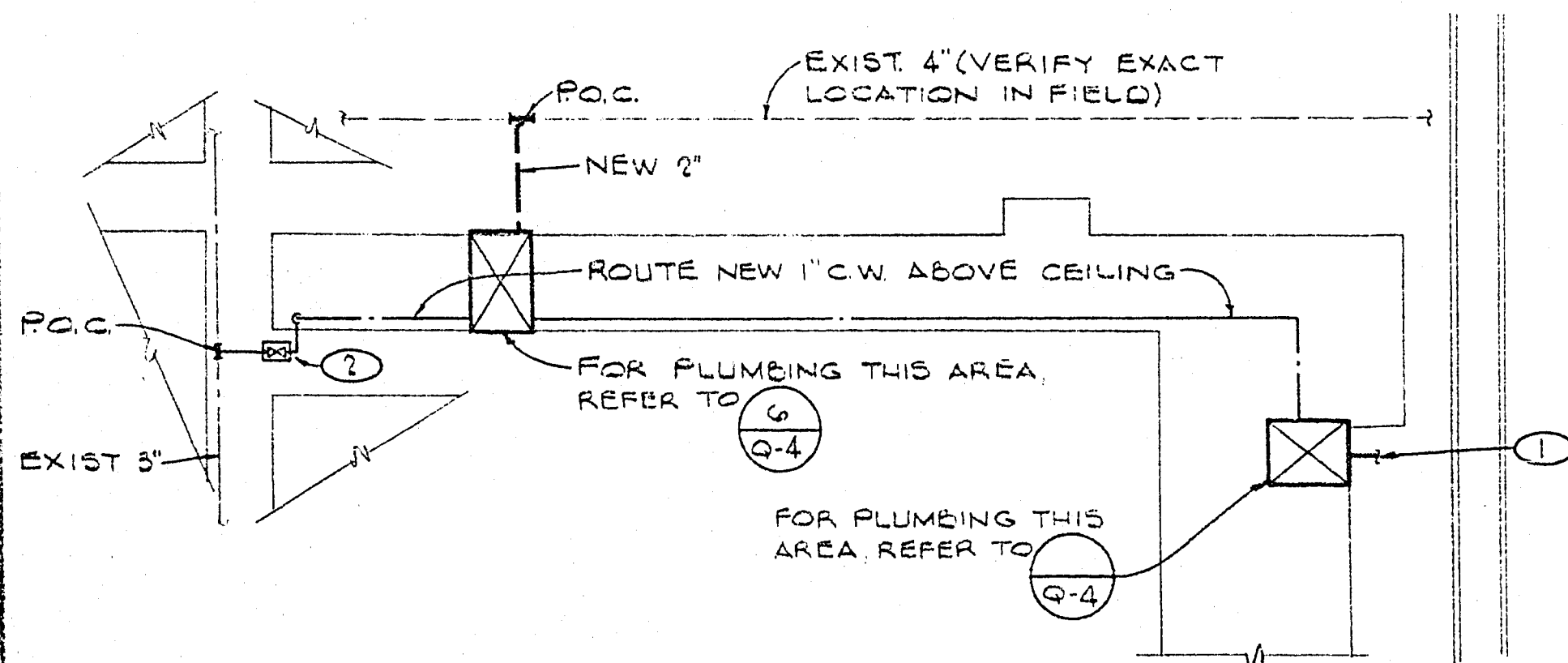
5 PARTIAL PLOT PLAN Q-2 SCALE: 1/8" = 1'-0"
