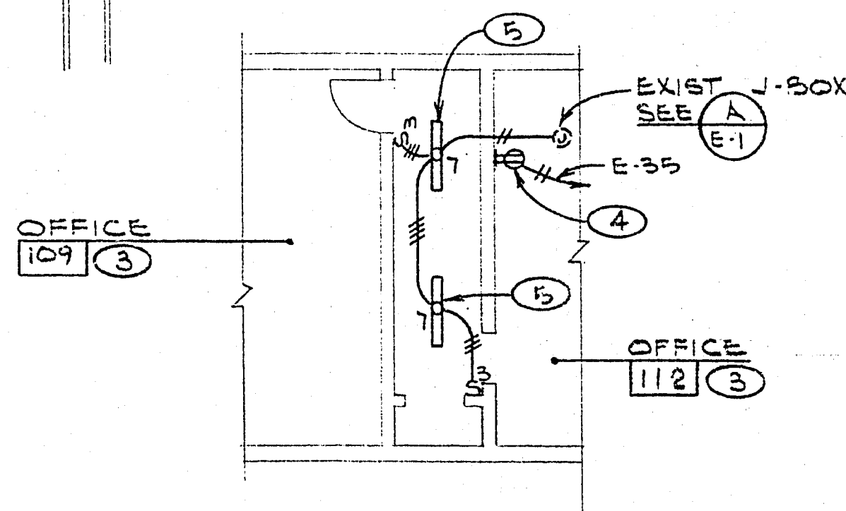
7 ELECT. PART PLAN Q-2 SCALE: 1/8" = 1'-0"
