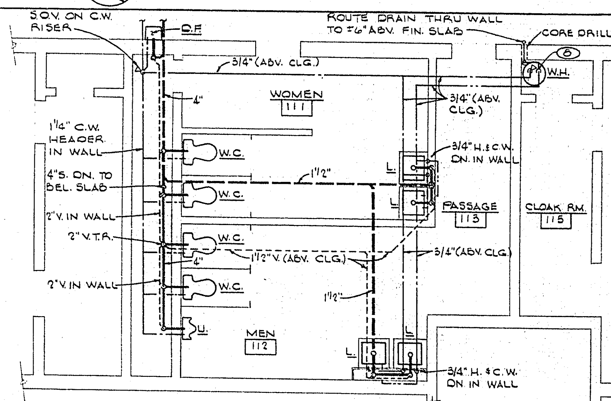
PLUMBING PART PLAN (C) 1/4" = 1'-0"
