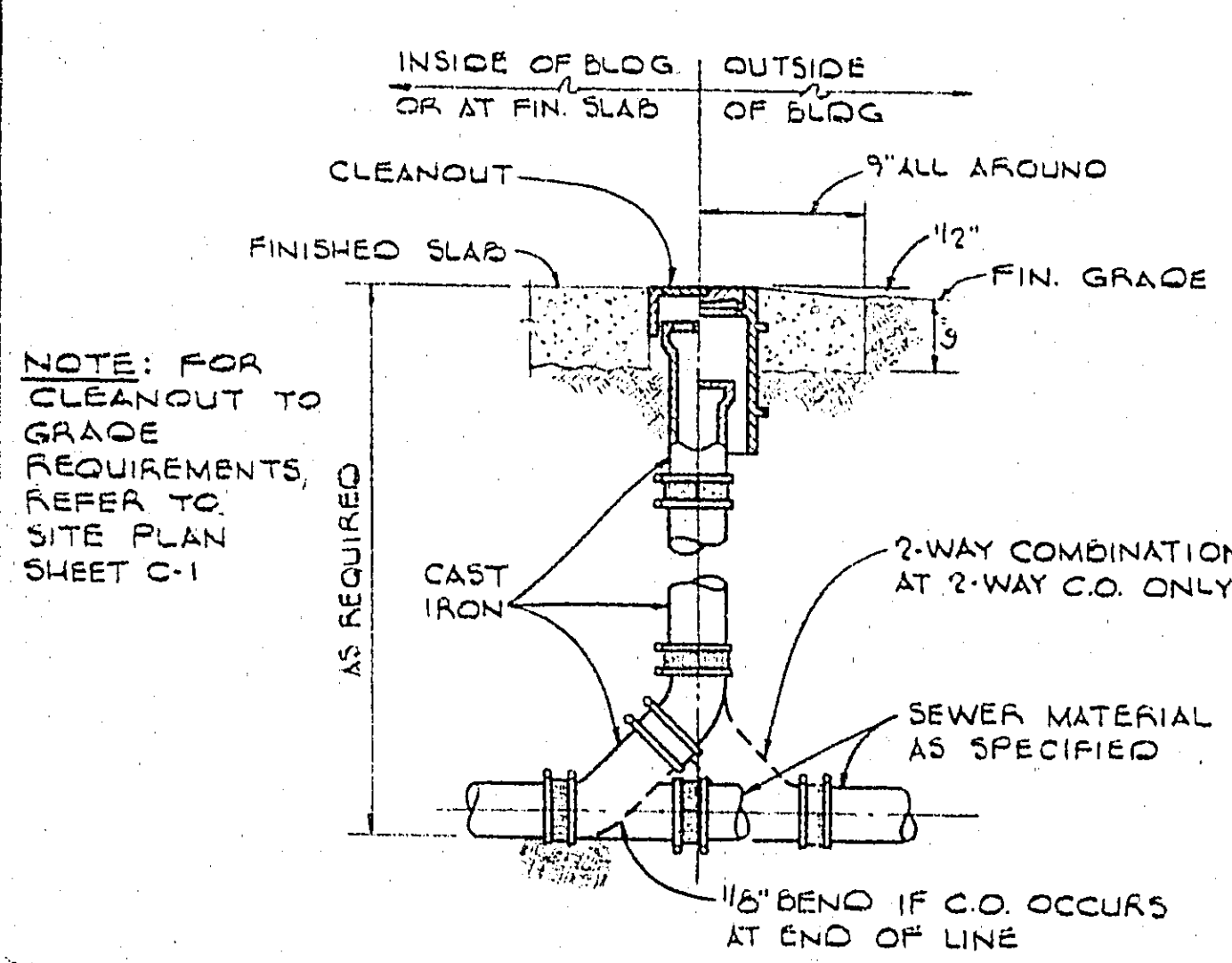
CLEANOUT DETAIL (I) NO SCALE
