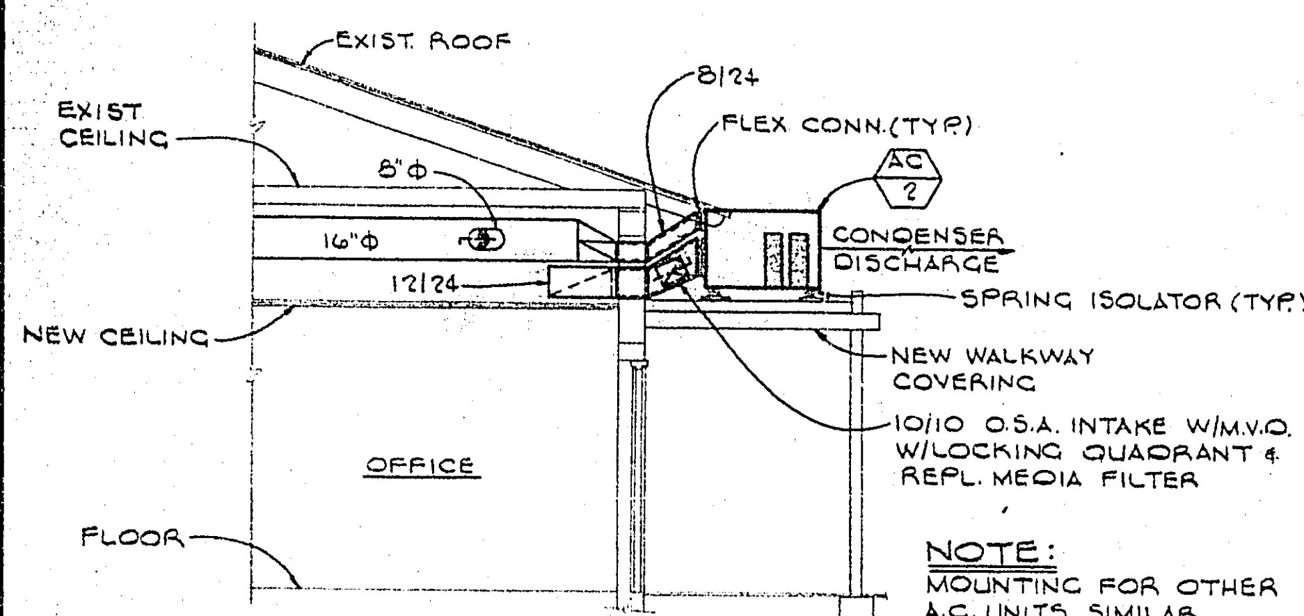
SECTION (B) 1/4" = 1'-0"
