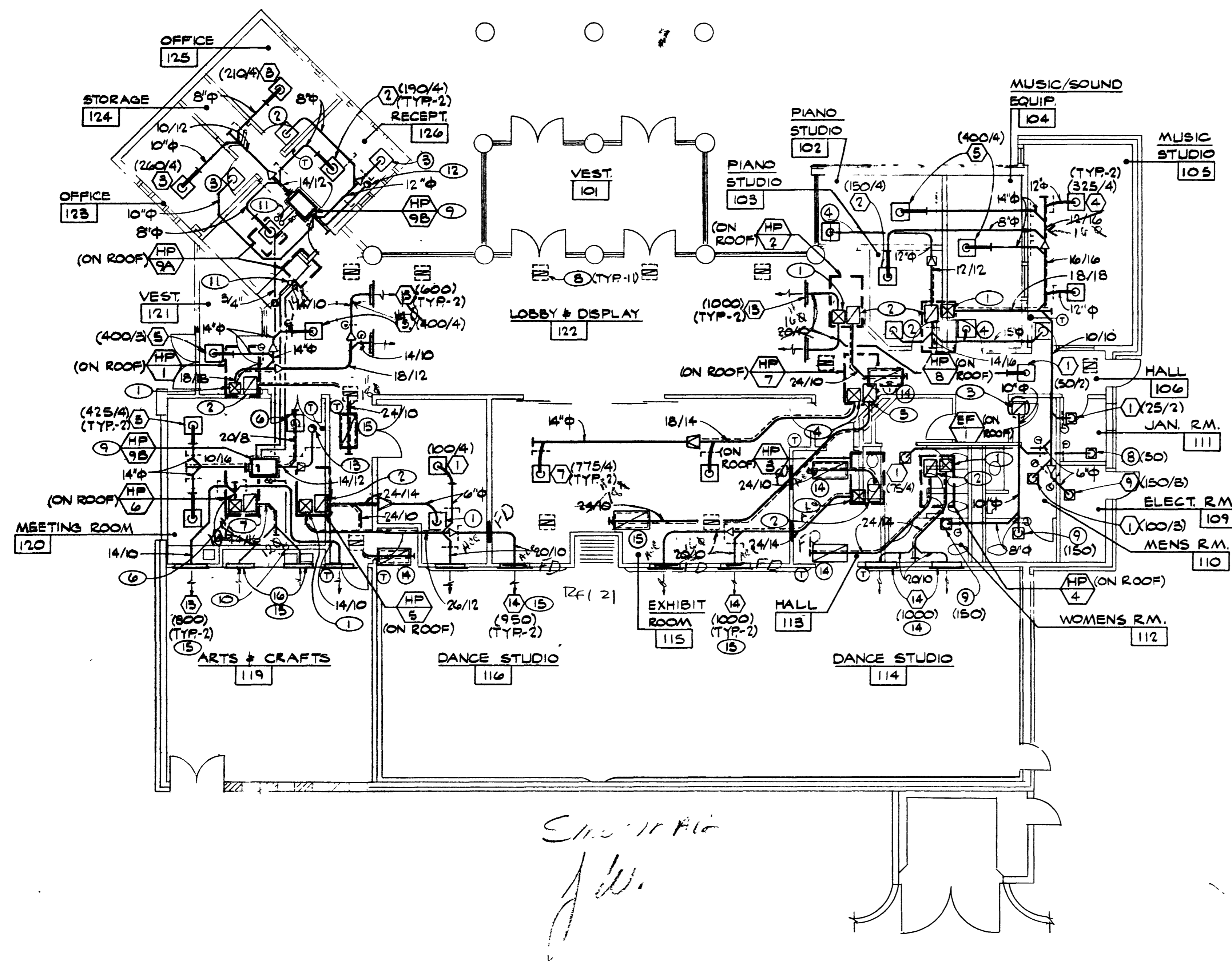
AIR CONDITIONING FLOOR PLAN SCALE: 1/8"=1'-0"
