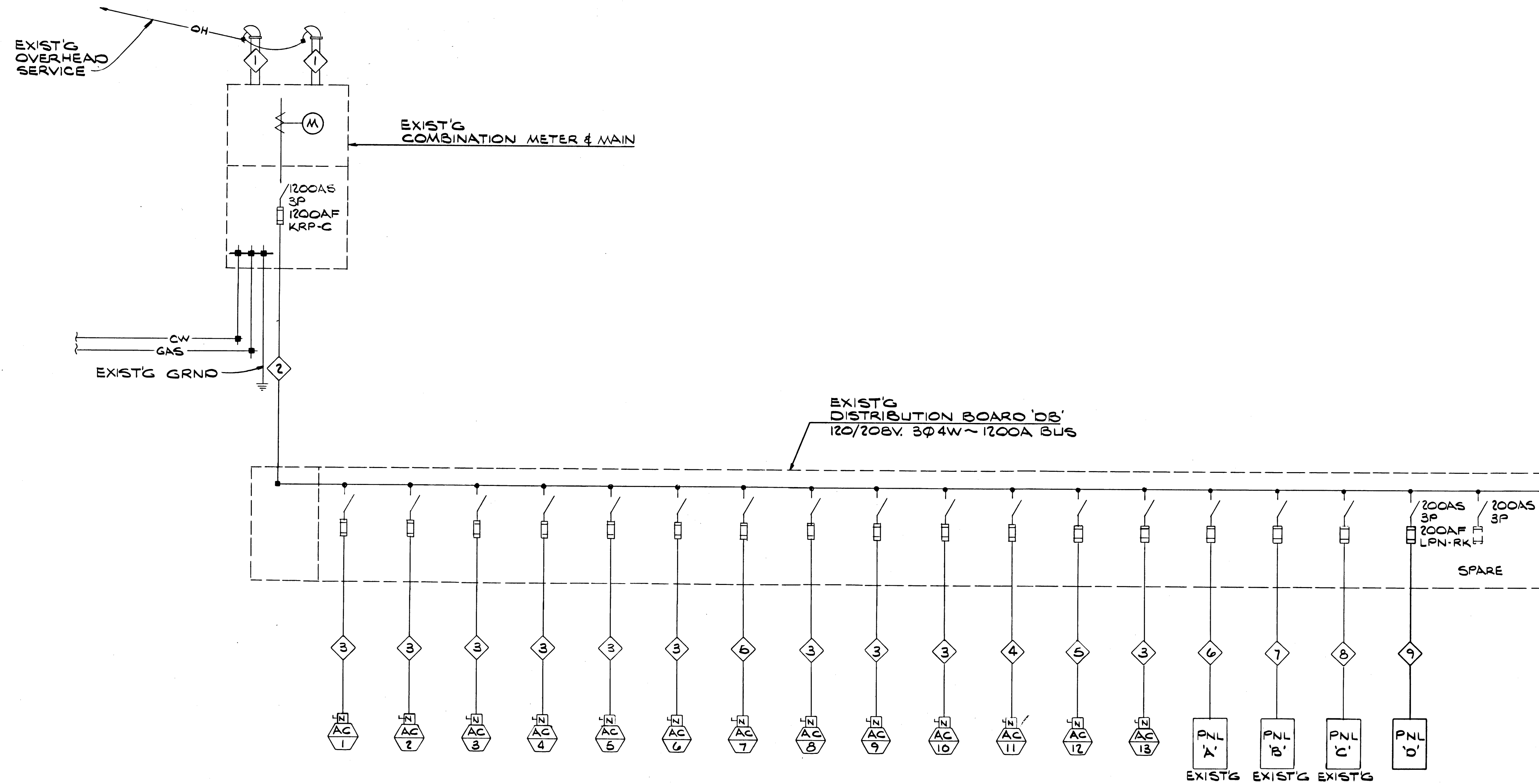
SINGLE LINE DIAGRAM
