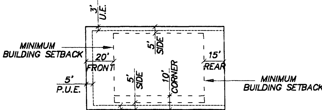
TYPICAL BUILDING SETBACK P.U.E. & U.E. N.T.S
