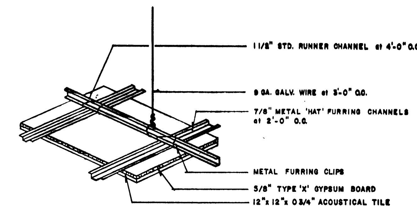
CEILING SUSPENSION DETAIL
