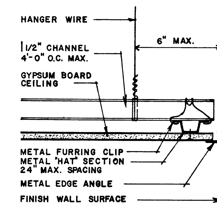
SUSPENDED GYP. BOARD CEILING
