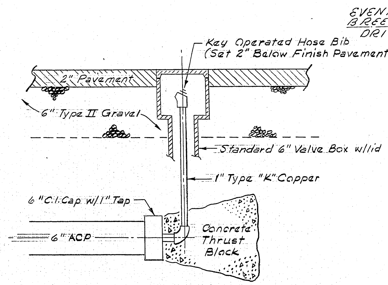
BLOWOFF DETAIL No Scale
