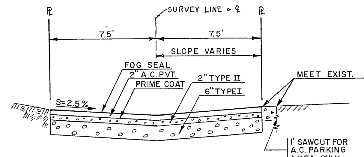
SECTION "A"-A" SCALE: 1" = 4' HOR. 1" = 2' VERT.
