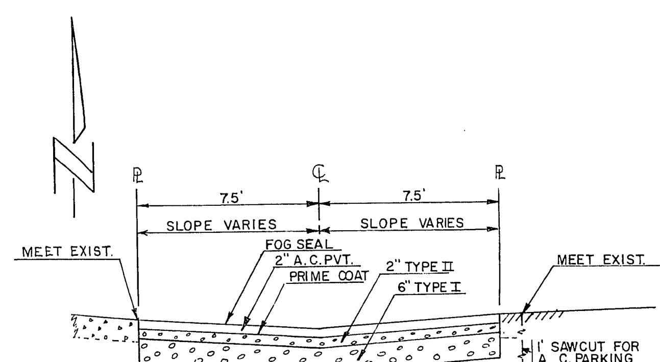
SECTION "B"-B" SCALE: 1" = 4' HOR. 1" = 2' VERT.
