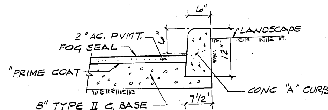
PAVEMENT & CURB DETAIL (NO SCALE)
